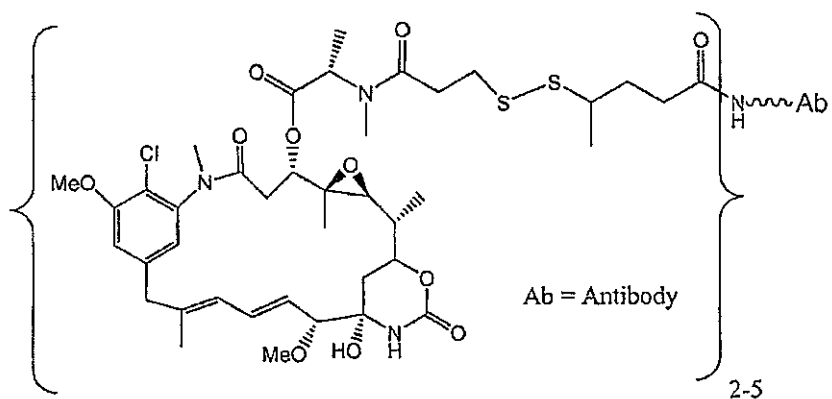
Ab-SPP-DM1
