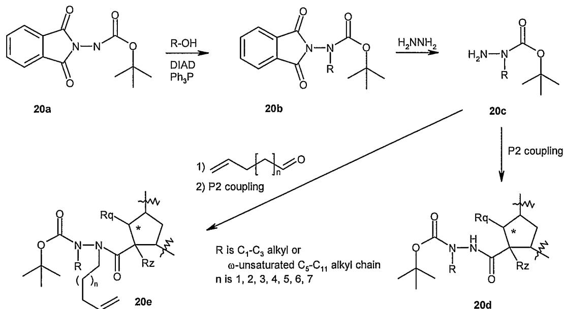
Scheme 20
