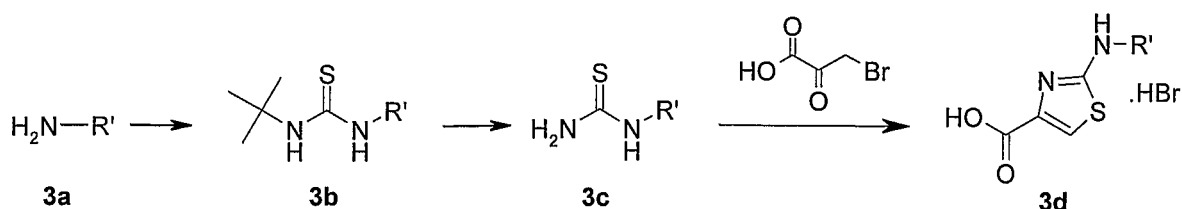
Scheme 3
