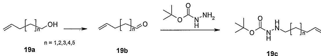
Scheme 19
