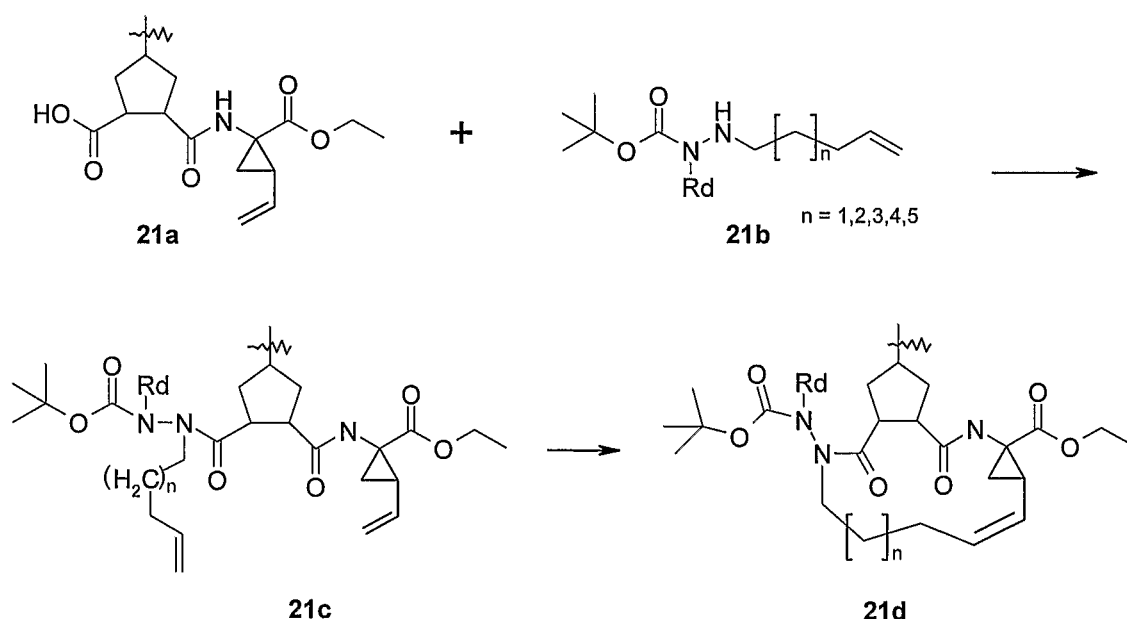
Scheme 21
