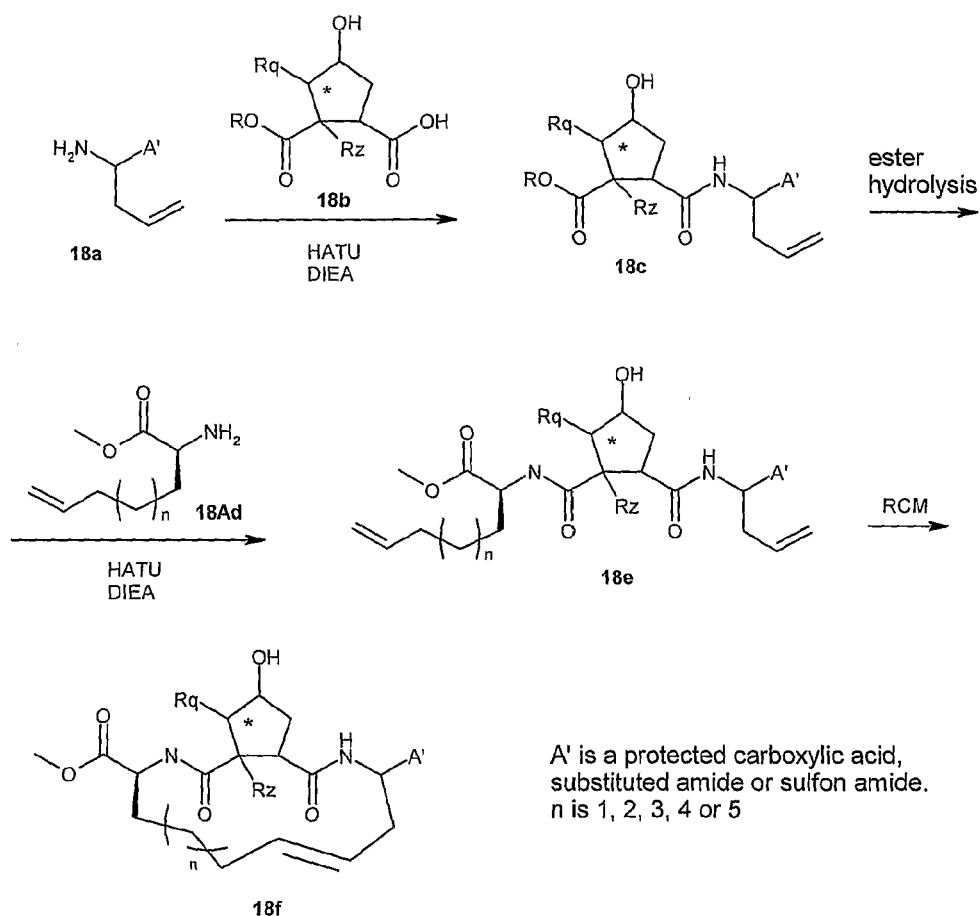
Scheme 18
