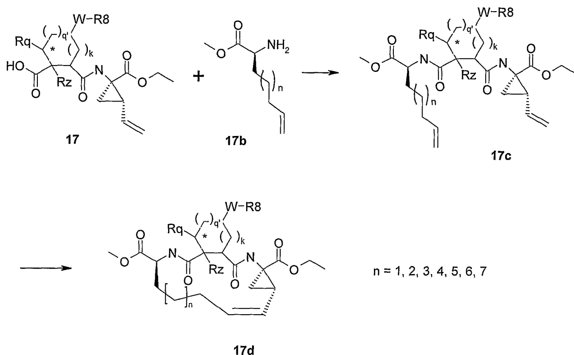
Scheme 17
