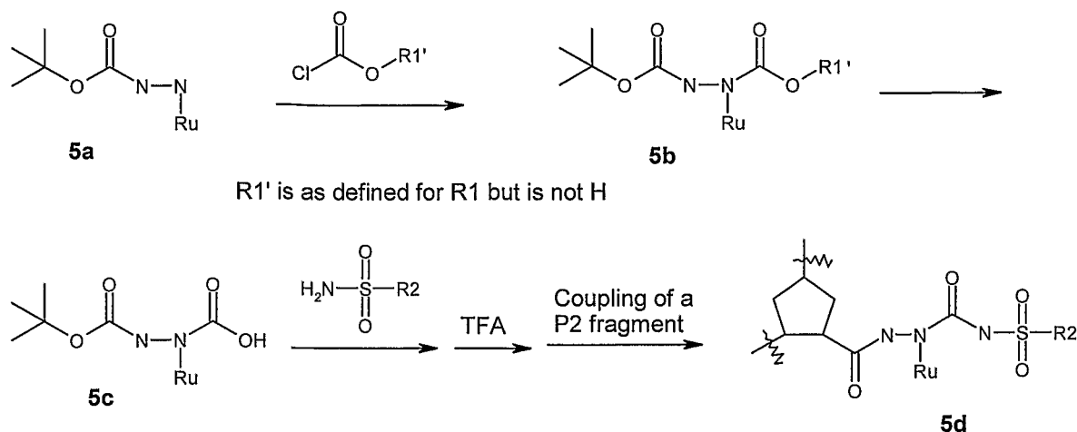
Scheme 5
