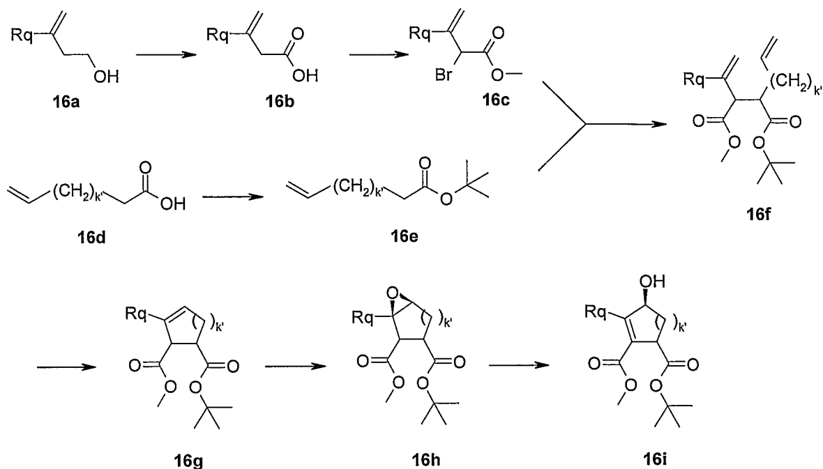
Scheme 11
