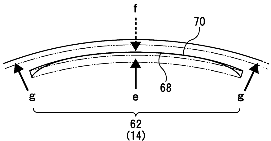
C [SHAPE CHANGE OF INNER CUT 62]
