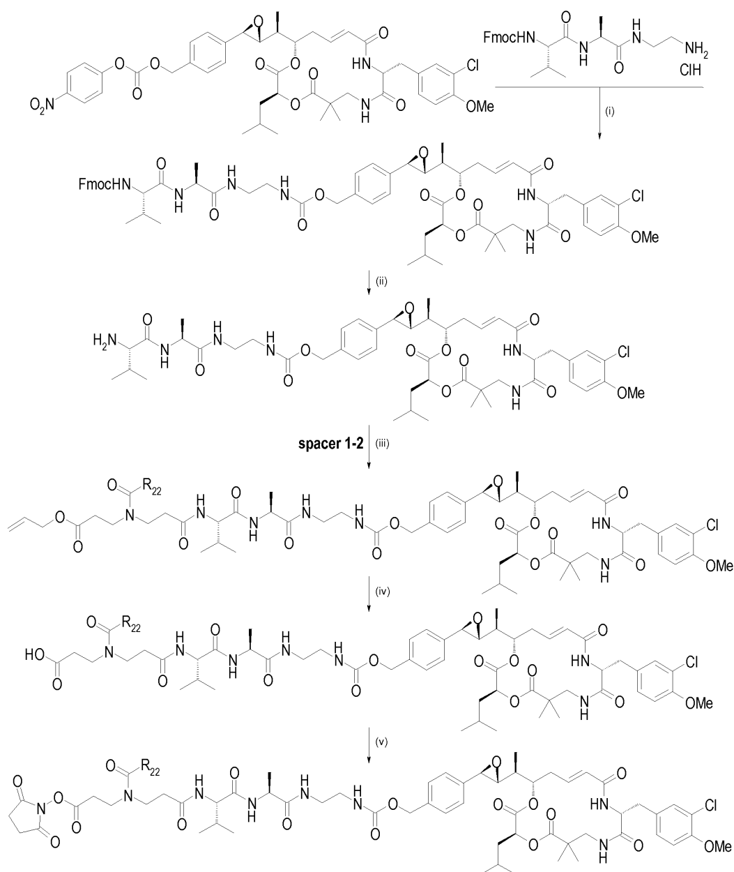
Scheme 15
