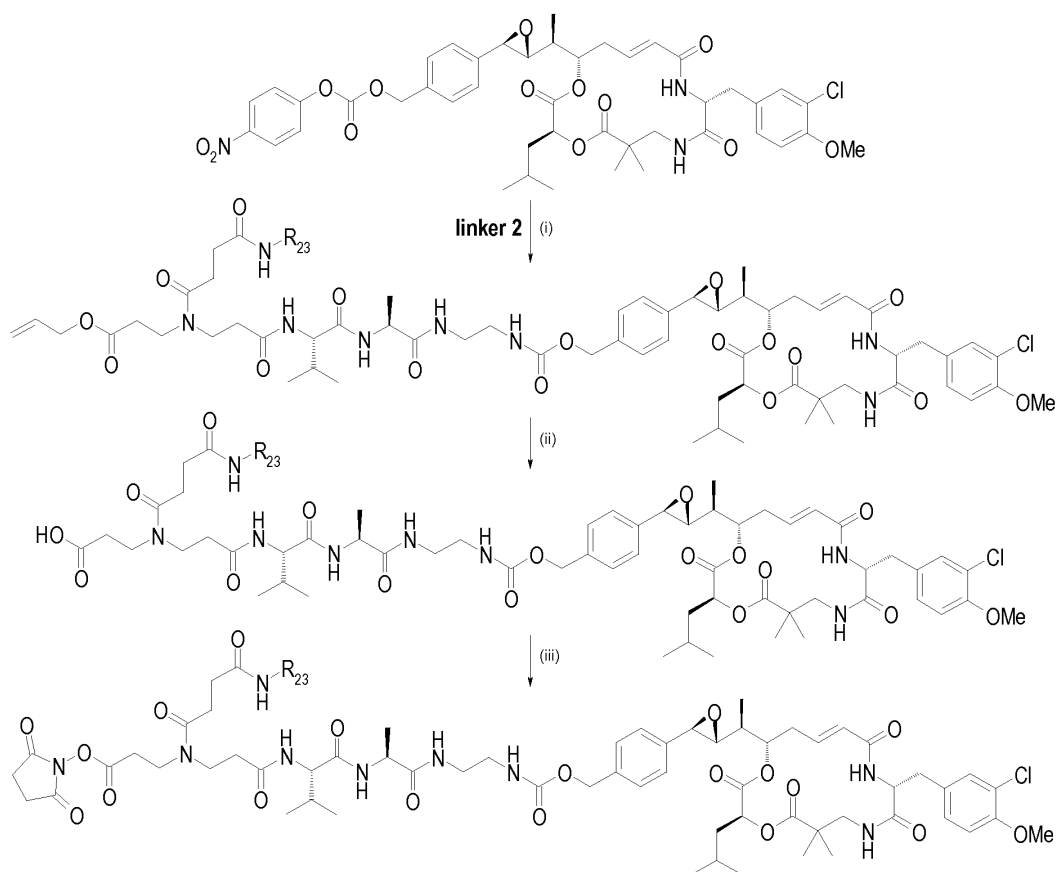
Scheme 16
