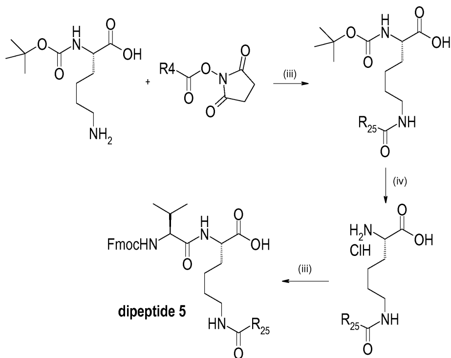
Scheme 6
