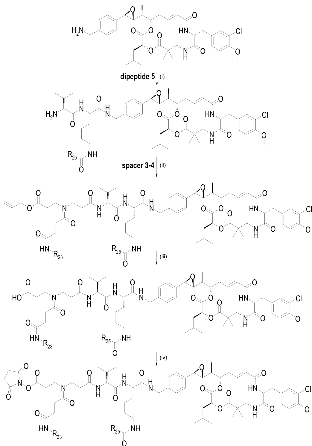
Scheme 13
