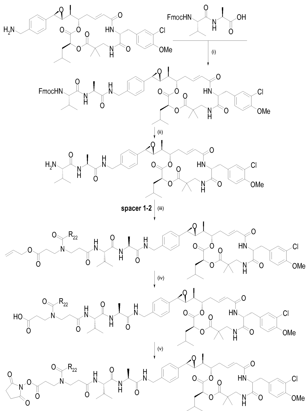
Scheme 8
