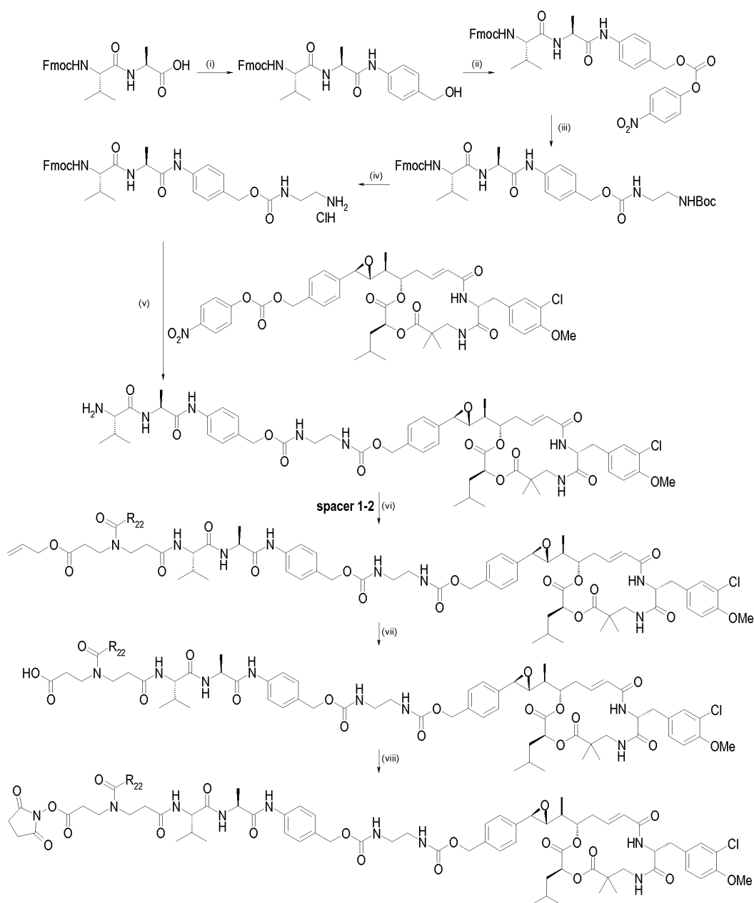
Scheme 17
