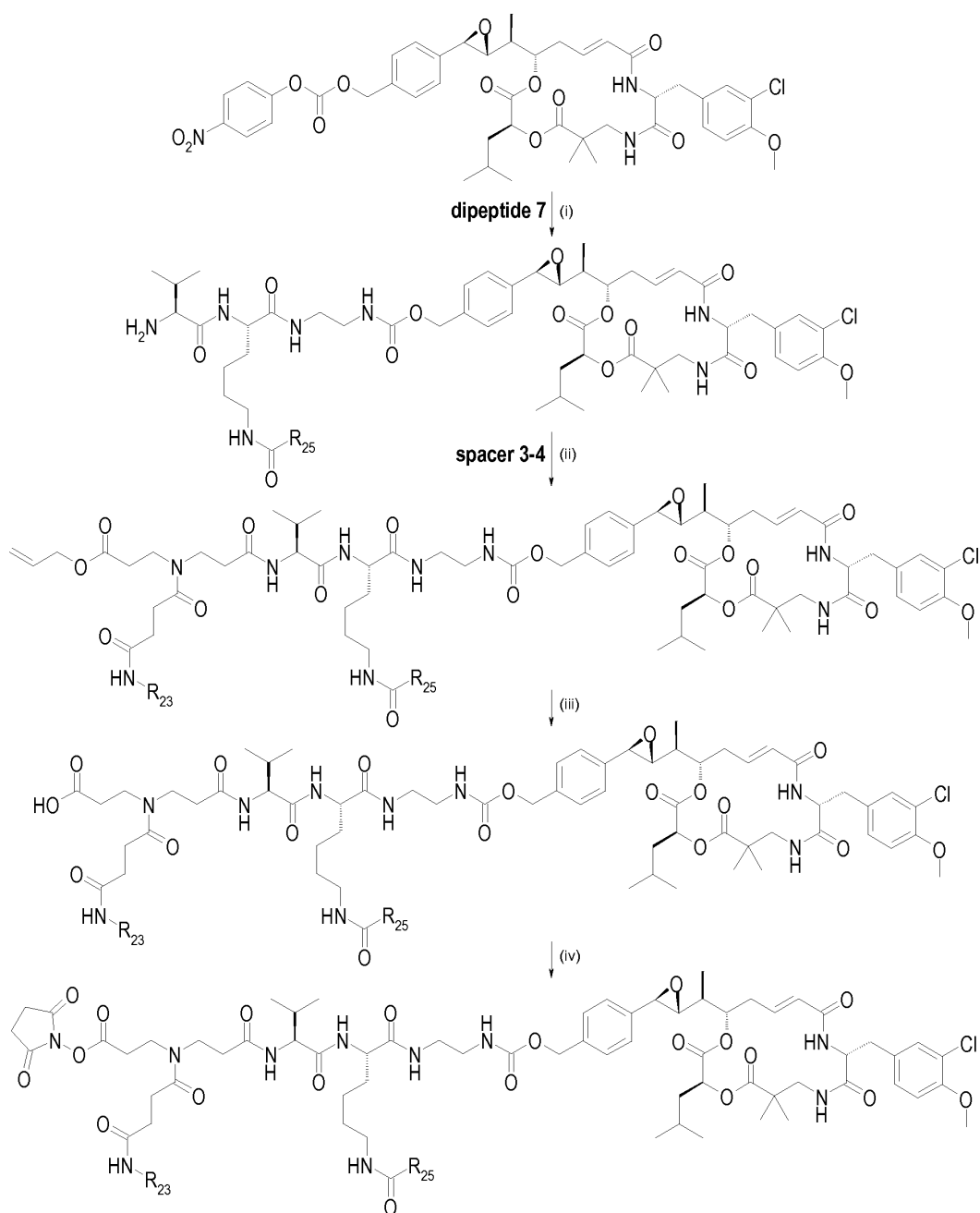
Scheme 20
