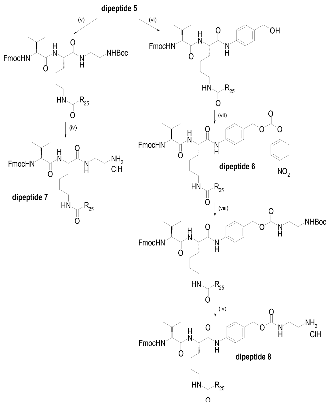
Scheme 7
