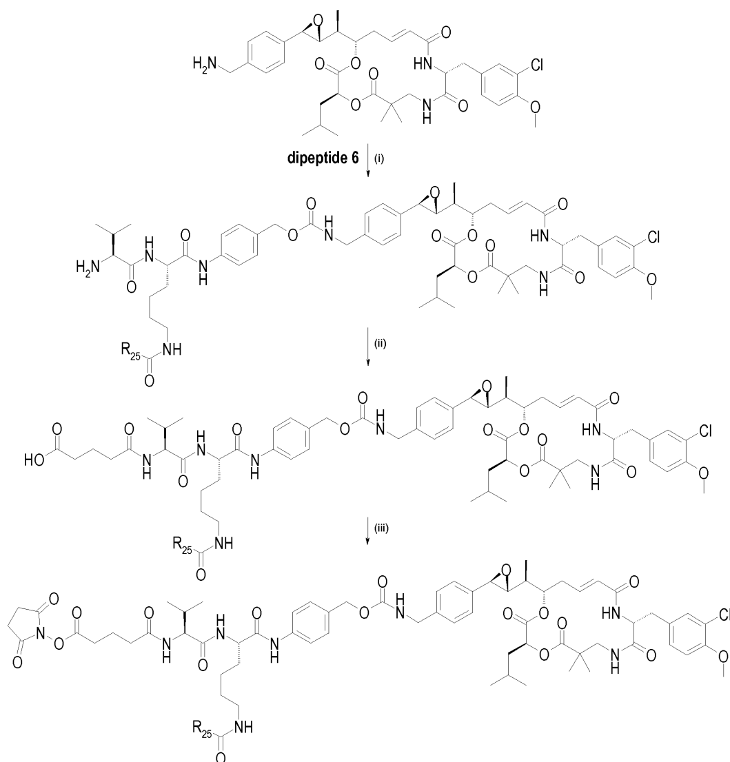
Scheme 12
