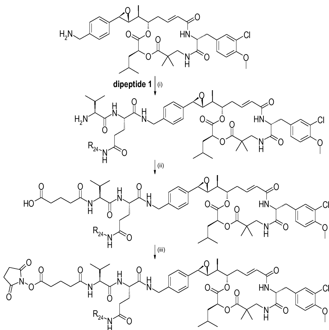
Scheme 11
