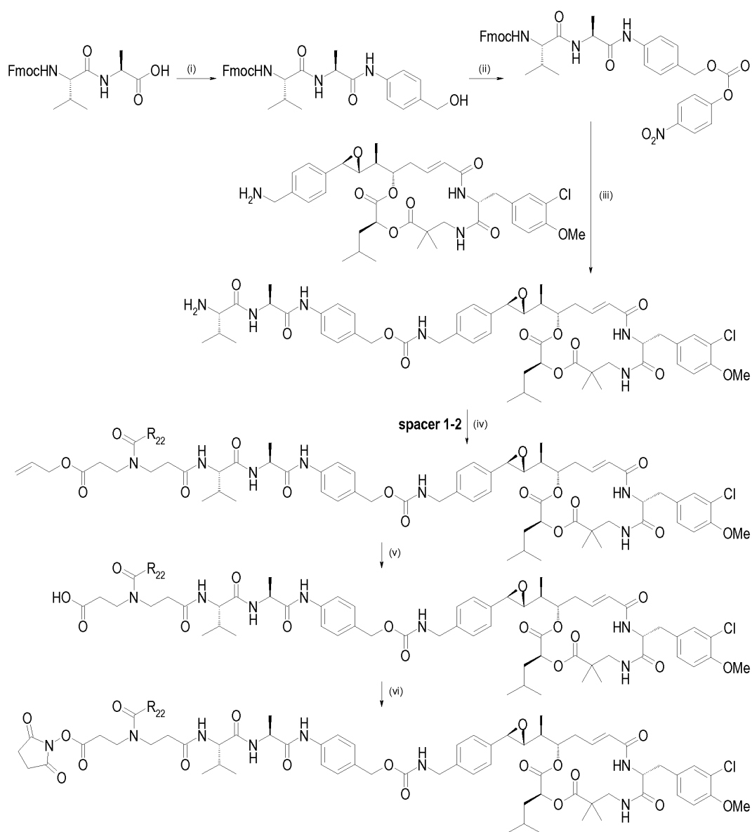
Scheme 10
