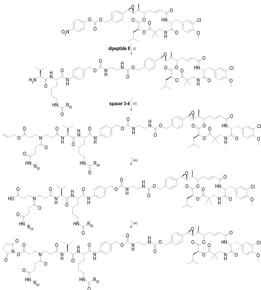
Scheme 21
