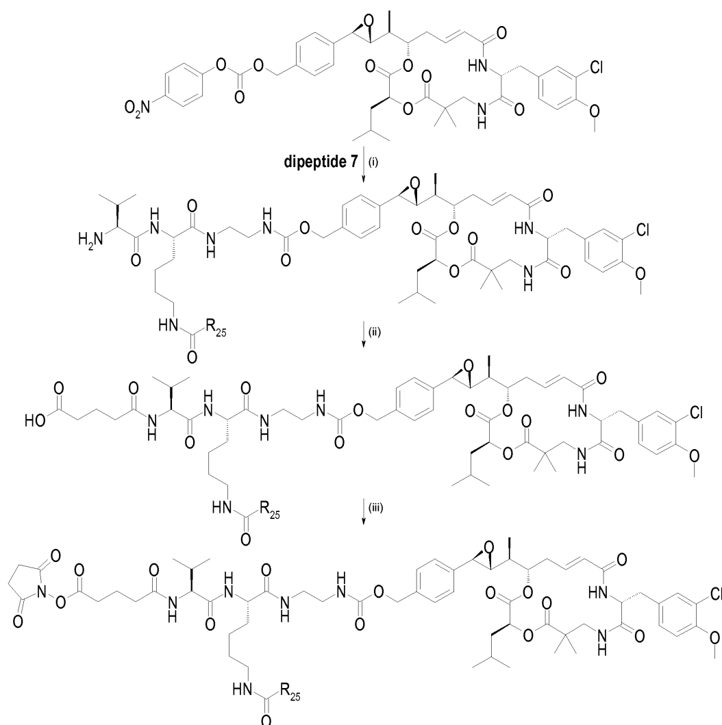
Scheme 18
