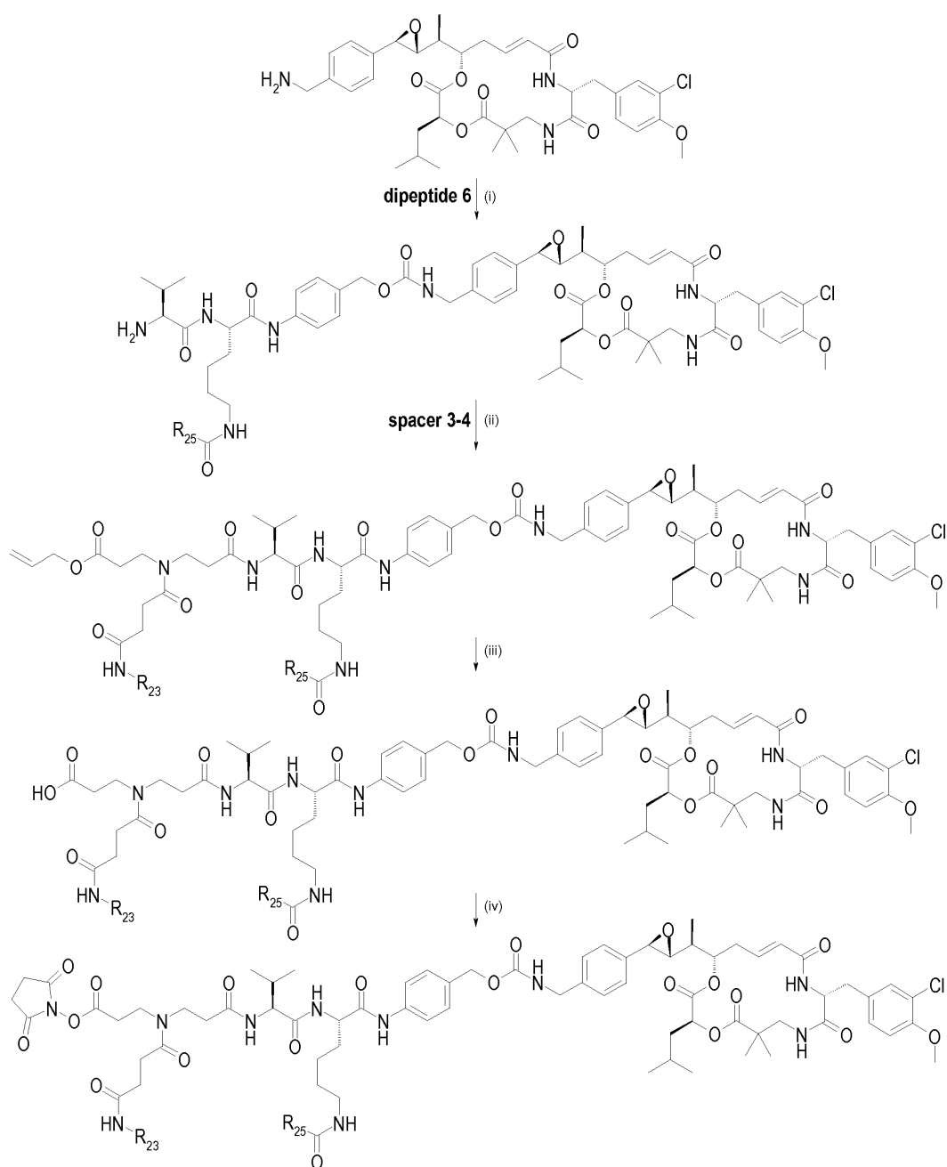
Scheme 14
