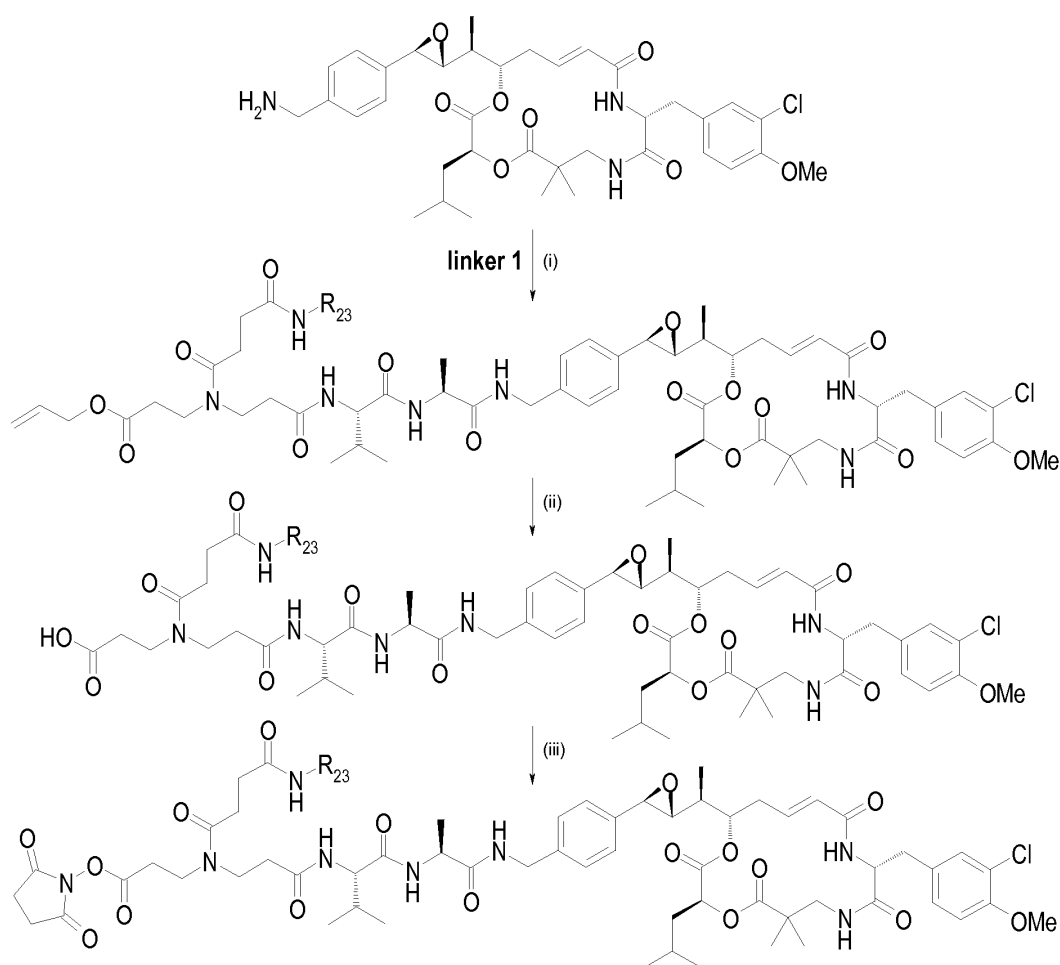
Scheme 9
