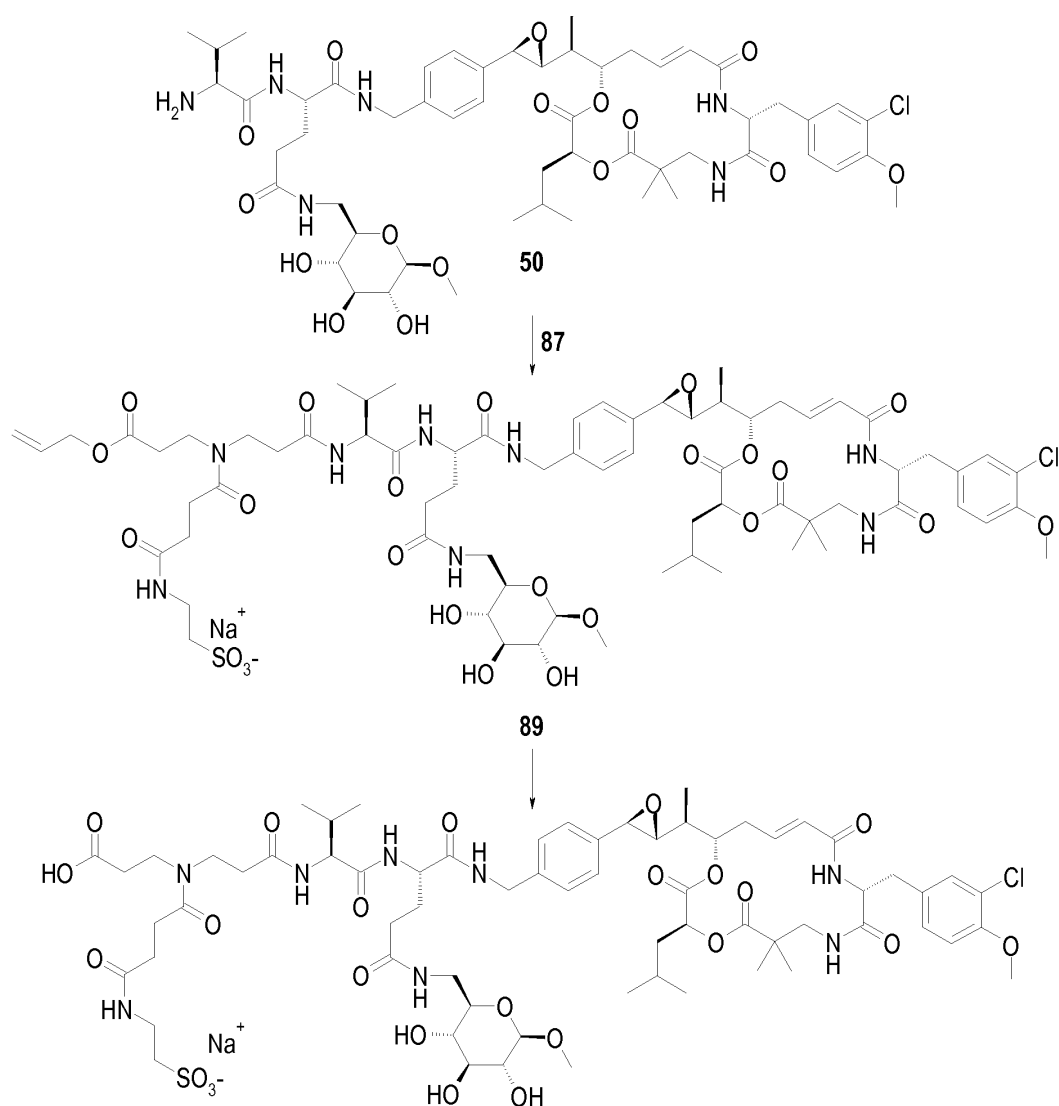
example 43
