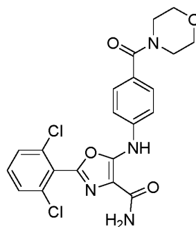
Compound B
