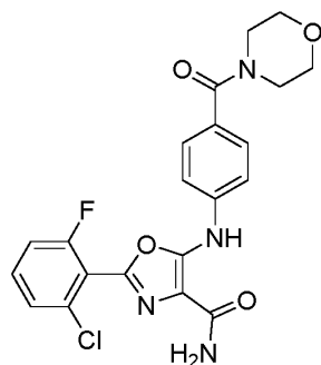
Compound A
