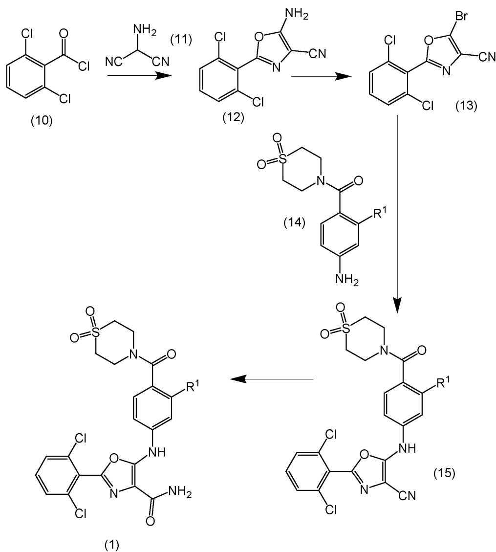
Scheme 1
