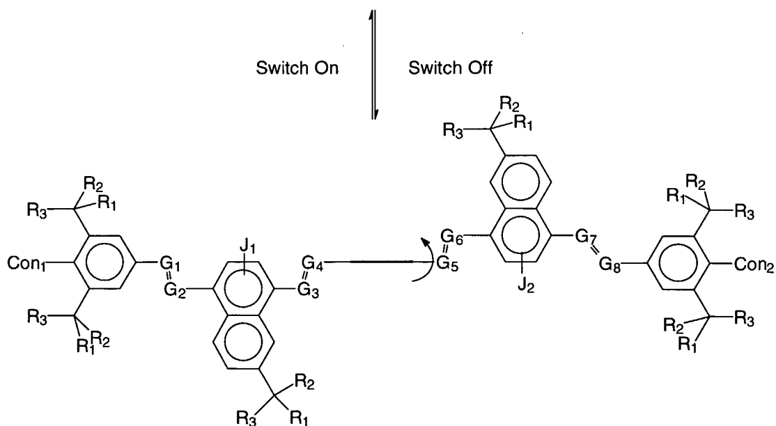
Off State (Optical State II)
