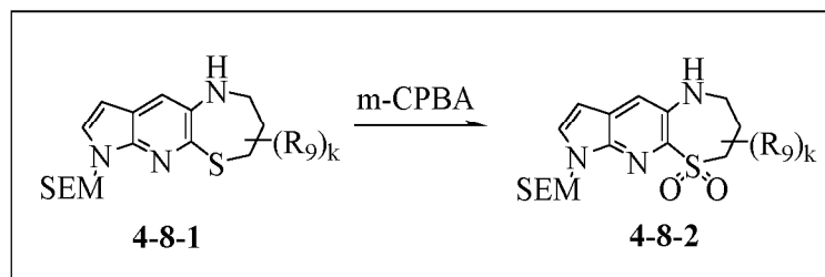
Scheme 4-8
