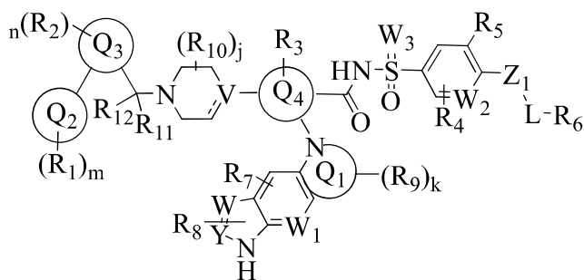
Formula (A)
