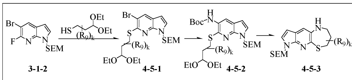
Scheme 4-5
