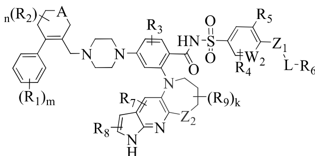
Formula (B)
