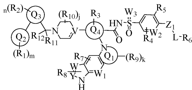
Formula (A)
