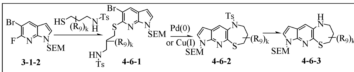
Scheme 4-6
