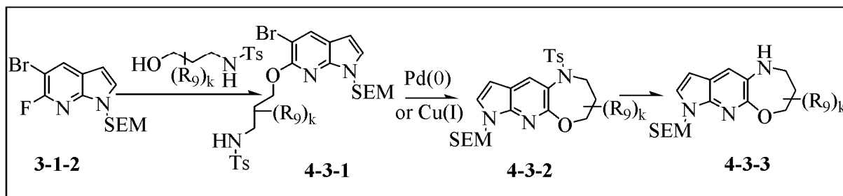
Scheme 4-3
