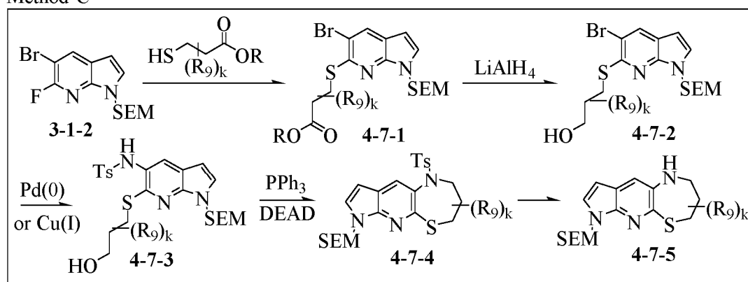
Scheme 4-7
