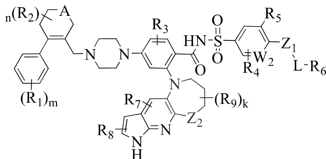
Formula (B)
