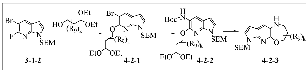
Scheme 4-2
