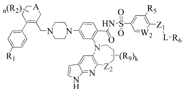
Formula (C)
