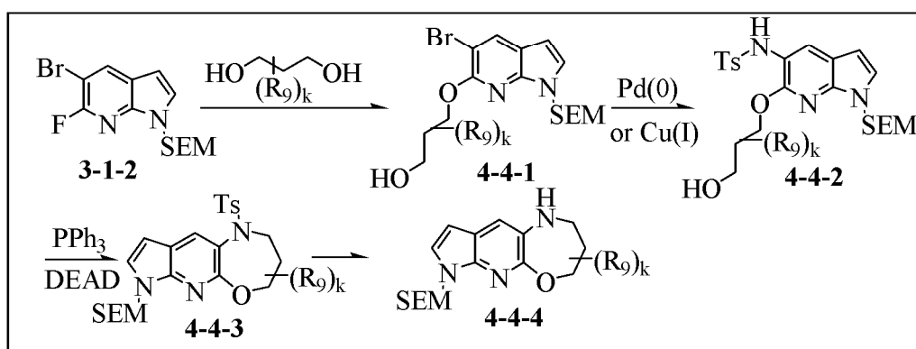
Scheme 4-4
