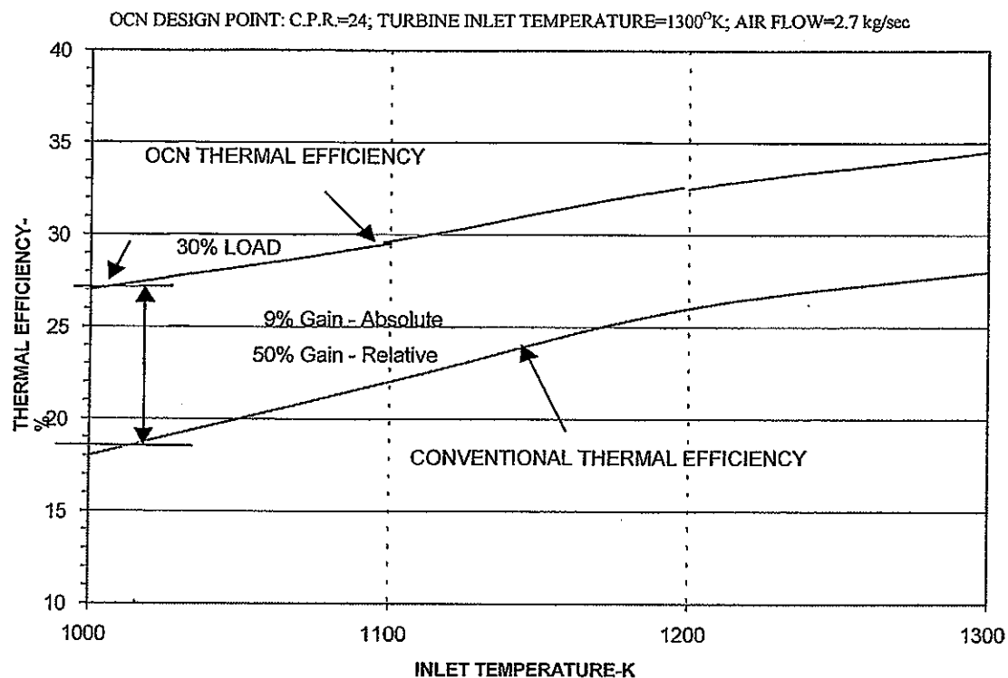
Fig. 9 -- EFFECT OF PART LOAD ON THERMAL EFFICIENCY
