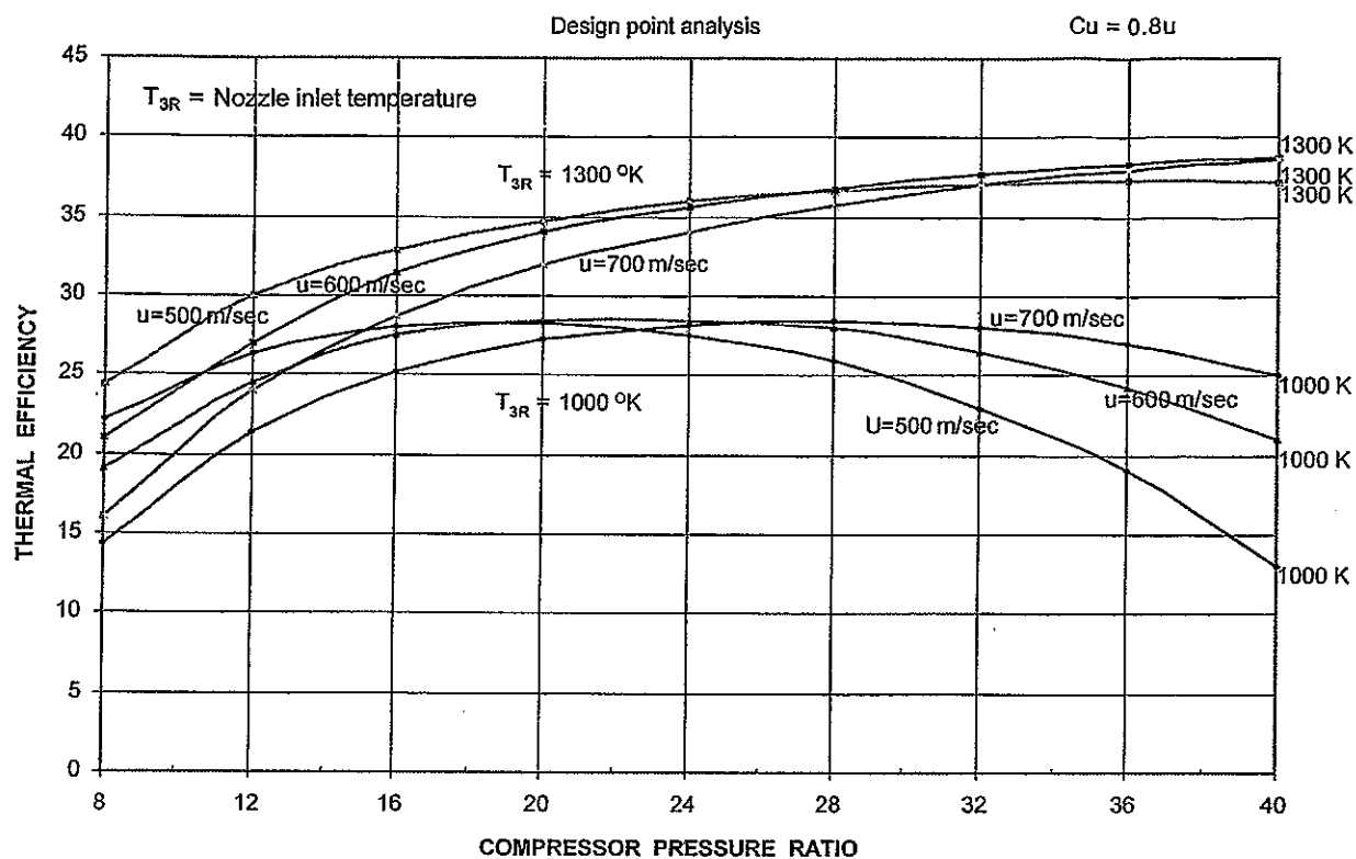
Fig 3. O.C.N THERMAL EFFICIENCIES
