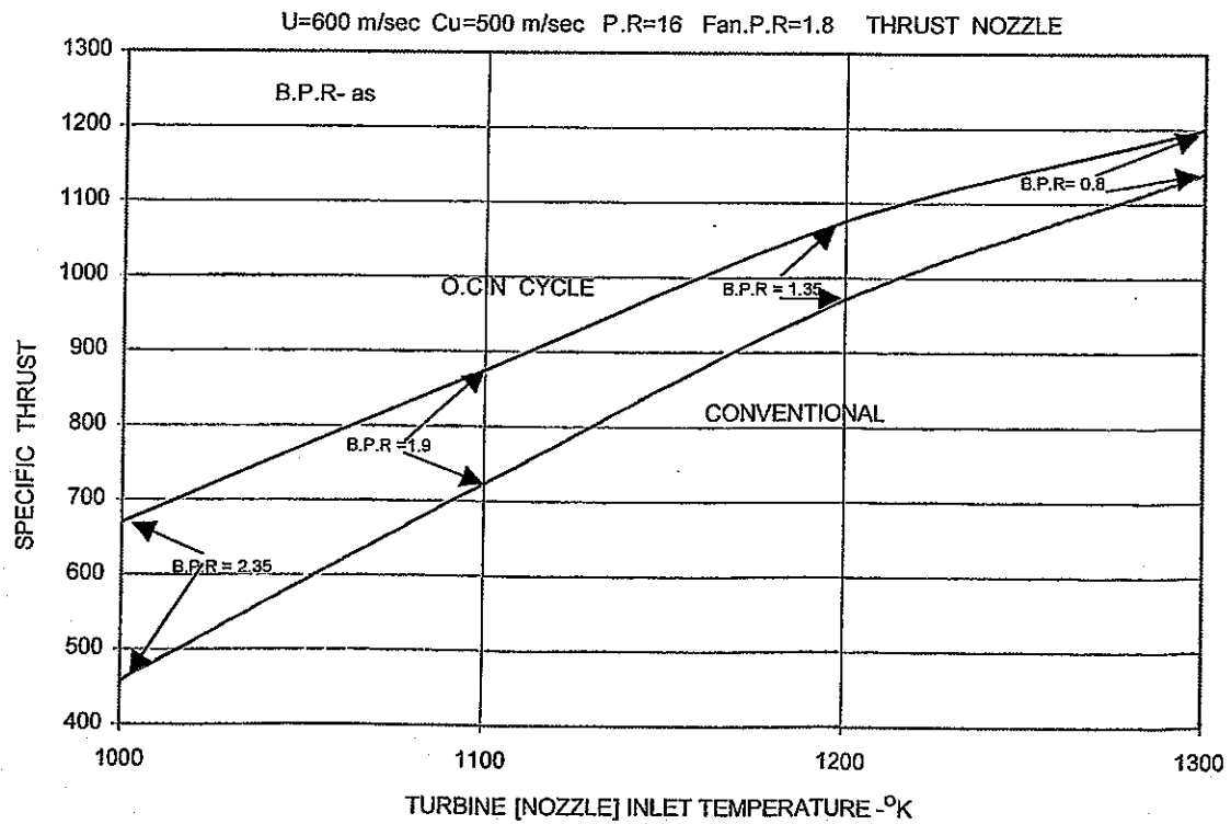
Fig 8. O.C.N TURBOFAN THRUST
