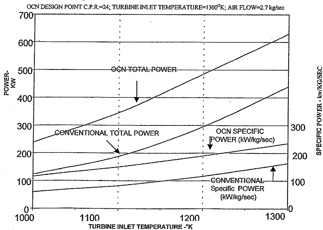
Fig. 10 EFFECT OF PART LOAD ON POWER
