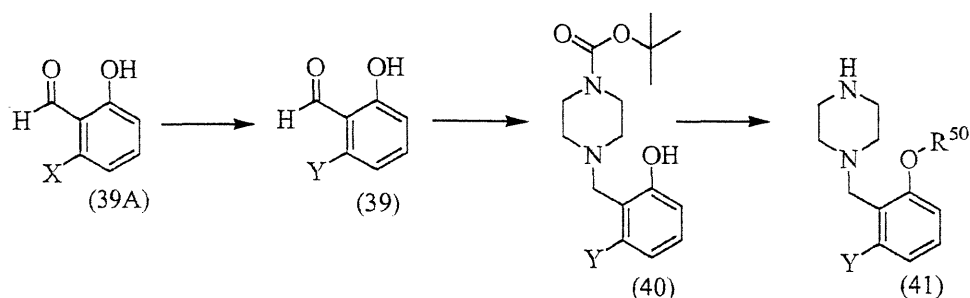
SCHEME 10
