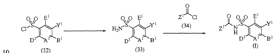
SCHEME 8
