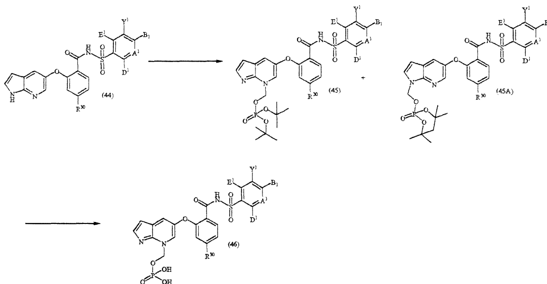
SCHEME 13
