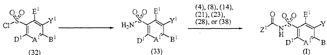
SCHEME 7
