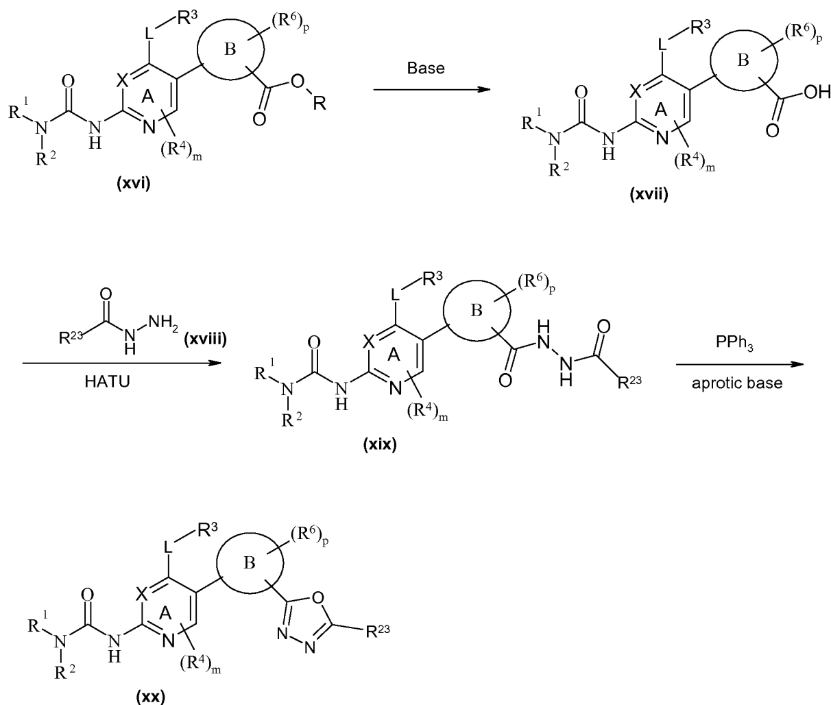
Scheme VII
