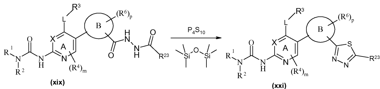
Scheme VIII
