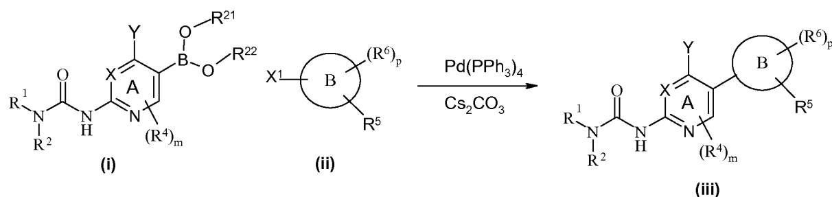
Scheme I
