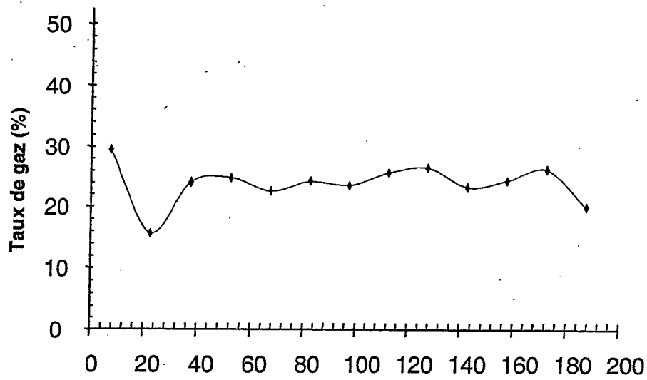
Figure 4b) Radial profile of the gas ratio in the bed [x-axis of the graph] column radius (mm) [y-axis of the graph] gas ratio (%)
