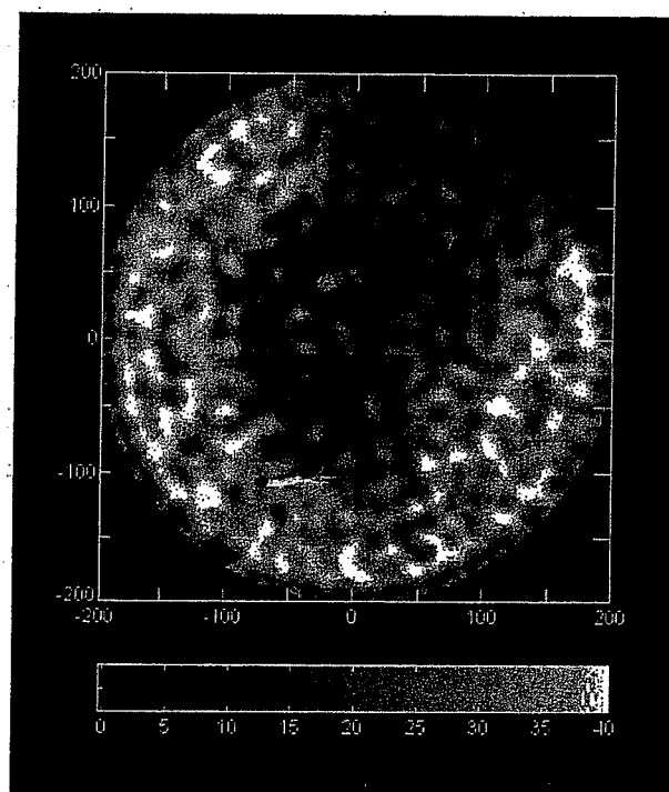
Figure 5a) 2D image of the gas ratio in the bed
