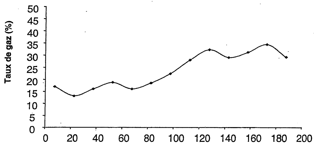
Figure 5b) radial profile of the gas ratio in the bed
