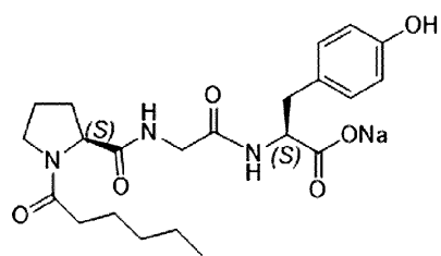
Compound I-7
