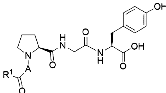
Formula I-Acid,
