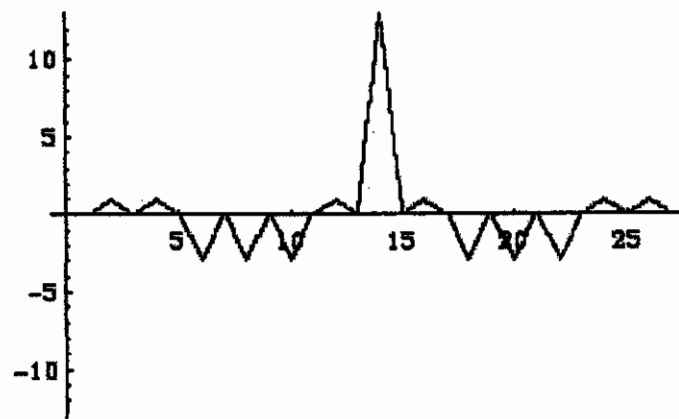
Autocorrelation of A
