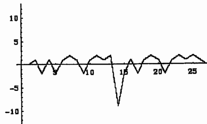
Inter-correlation of A and B
