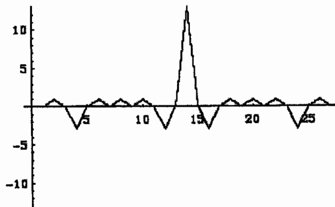
Autocorrelation of B
