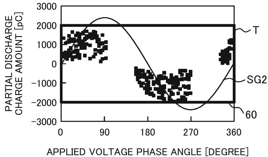
(A) PARTIAL DISCHARGE CHARGE AMOUNT PHASE ANGLE DISTRIBUTION PATTERN T
