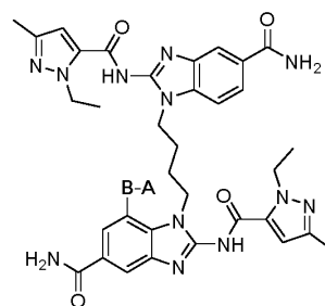
STING agonist 2
