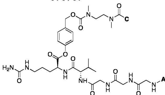
gly-gly-gly-Val-Cit-PAB
