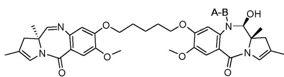
PBD
