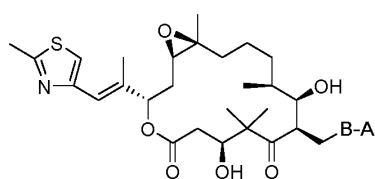
Epothilone B
