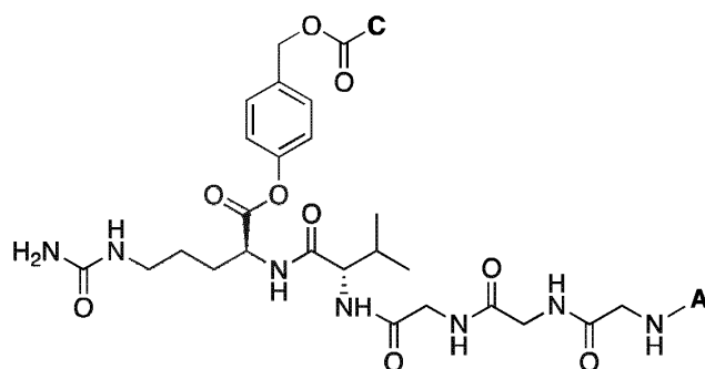
gly-gly-gly-Val-Cit-PAB
