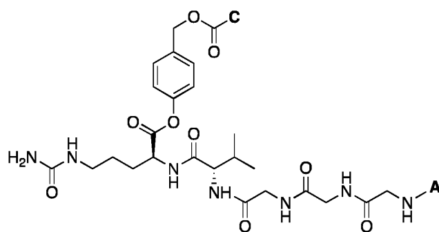
gly-gly-gly-Val-Cit-PAB
