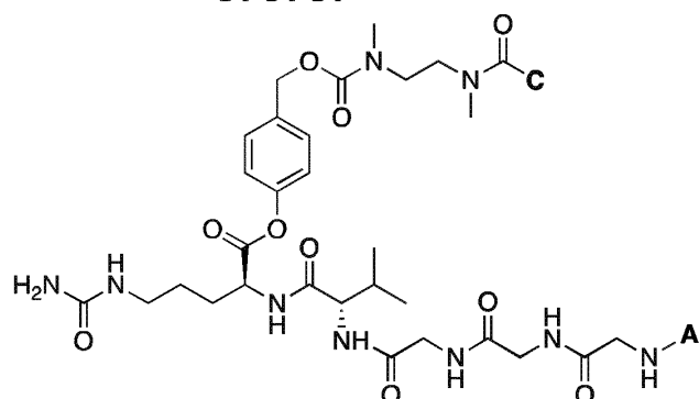
gly-gly-gly-Val-Cit-PAB
