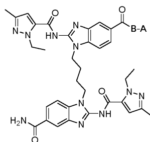
STING agonist 1
