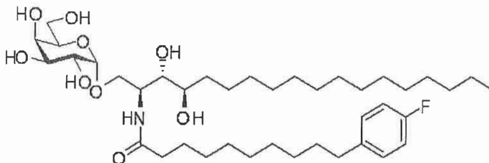
compound 7 (7DW8-5)
