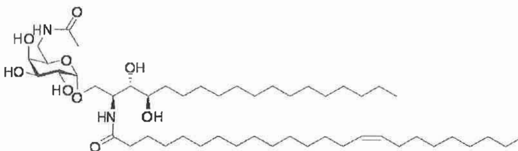
compound 5 (PBS-57)
