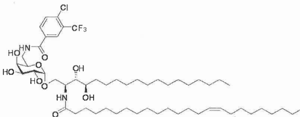
compound 6
