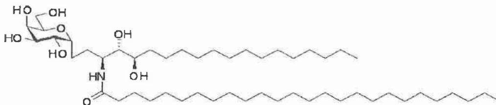
compound 2 (α-C-GalCer)
