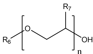
(Formula Va)
