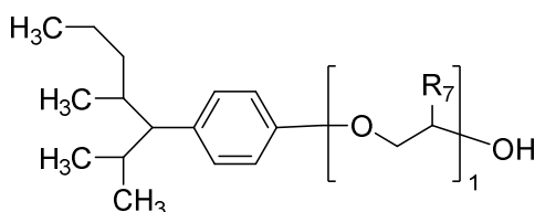
(Formula Vc)
