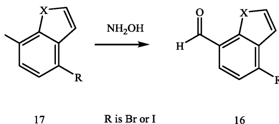
Scheme 14
