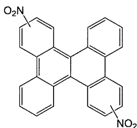
(NO 2 DBC-2)
