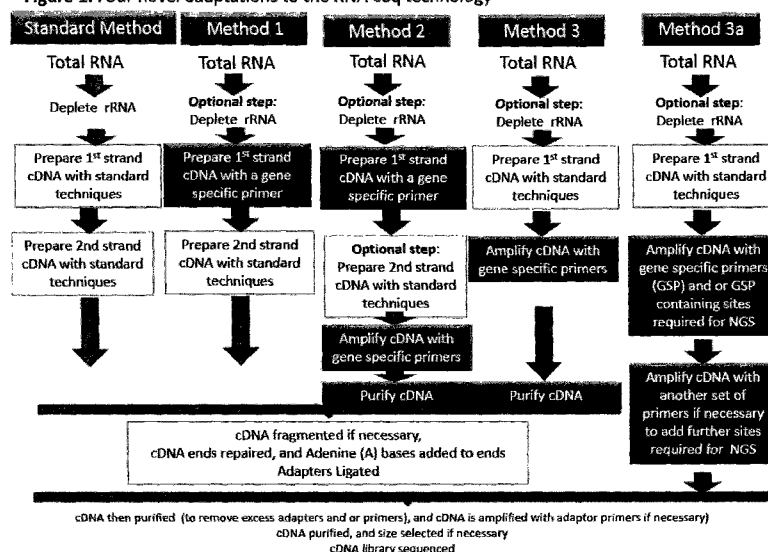
Figure 1: Four novel adaptations to the RNA-seq technology
