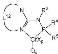
Structure GuCr2
