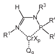
Structure NPFCr1
