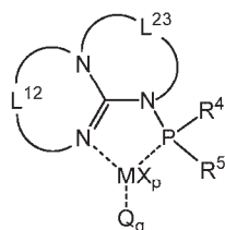
Structure GuMC4
