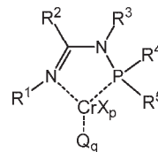
Structure NPACr1
