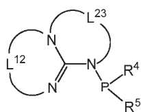
Structure Gu4
