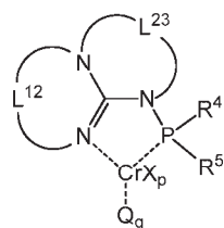
Structure GuCr4
