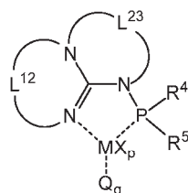
Structure GuMC5
