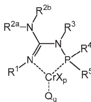
Structure GuCr1
