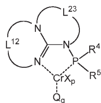
Structure GuCr5
