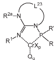
Structure GuCr3
