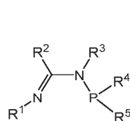
Structure NPA1
