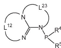
Structure Gu5
