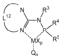
Structure GuMC2
