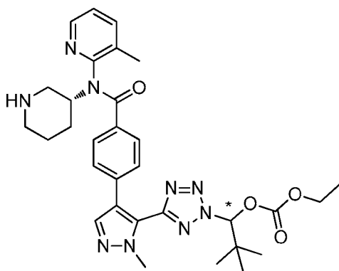
Diastereomer B
