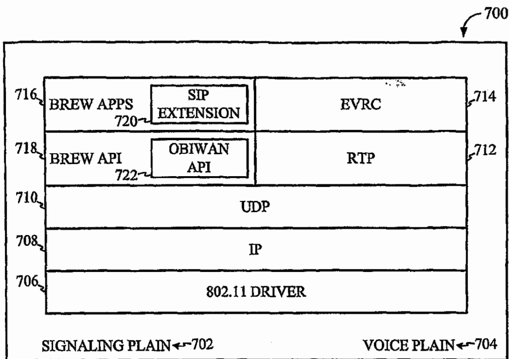
FIG. 7: WIRELESS TERMINAL PROTOCOL STACK BEFORE THE HANDOFF
