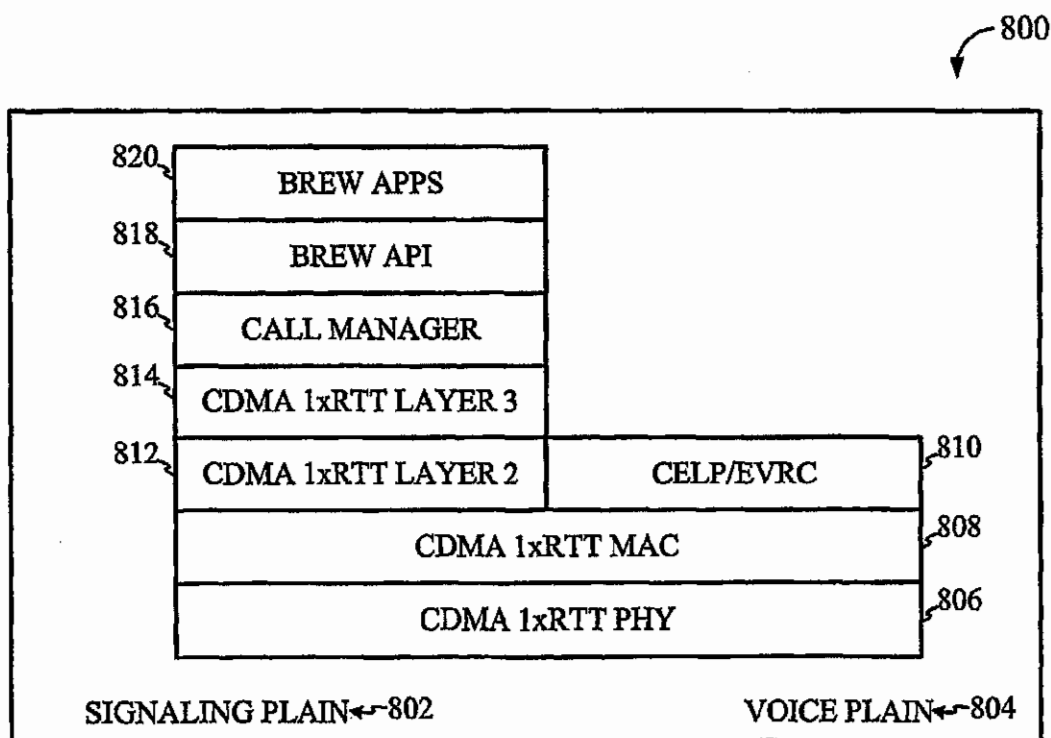
FIG. 8: WIRELESS TERMINAL PROTOCOL STACK AFTER THE HANDOFF
