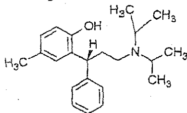
(R)-stereoisomer
