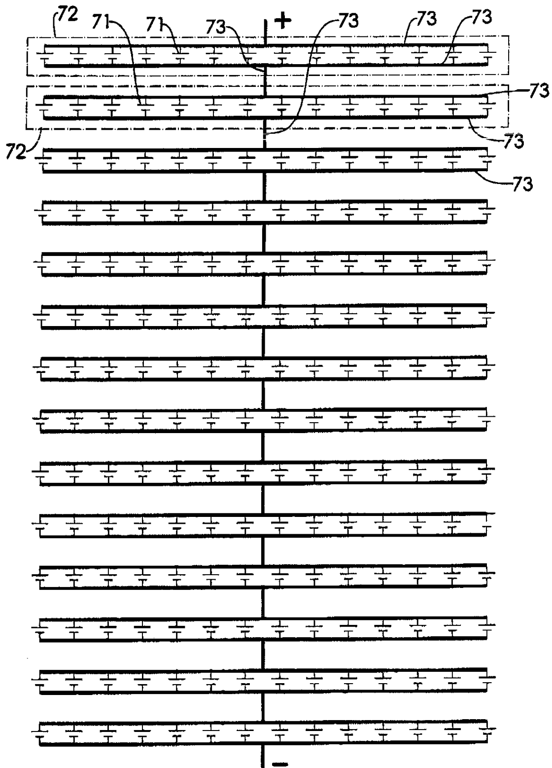
FIG.12 PRIOR ART
