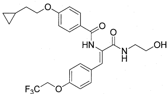
(13a) 4-(2,2,2-Trifluoroethoxy)benzaldehyde
