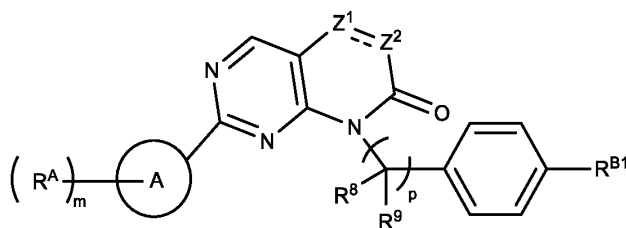
Formula (IIIc-1').
