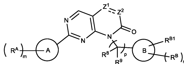
Formula (IIIa)
