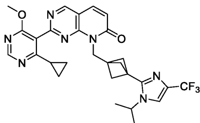
Compound 37
