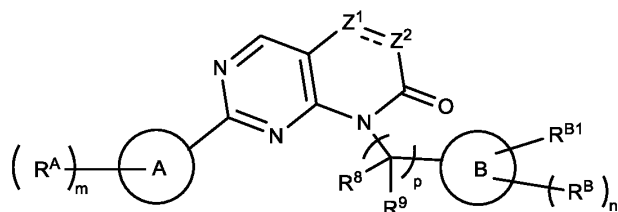
Formula (IIIa).
