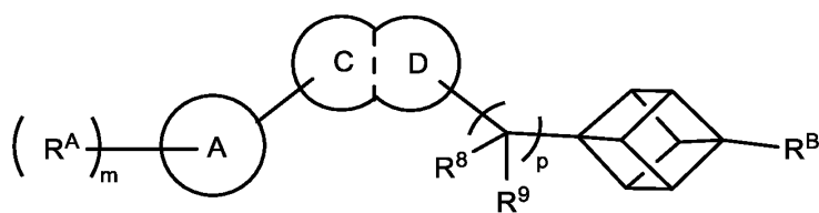
Formula (VI)
