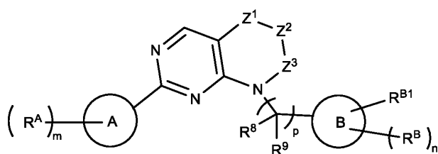
Formula (IIIb)
