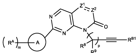
Formula (IIId').
