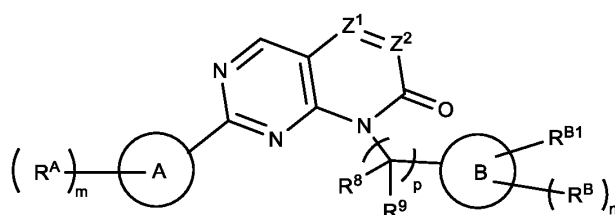
Formula (IIIa-1).
