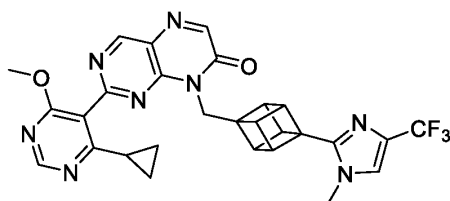
Compound 27
