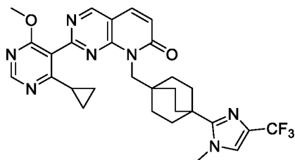
Compound 35
