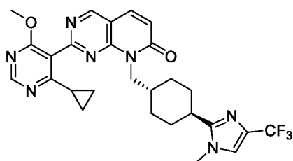
Compound 38
