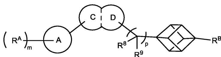
Formula (VI)
