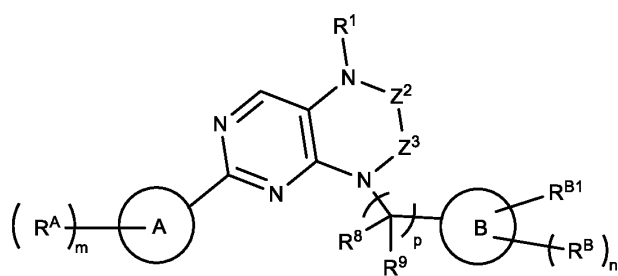
Formula (IIIb-2).
