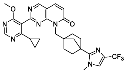
Compound 36
