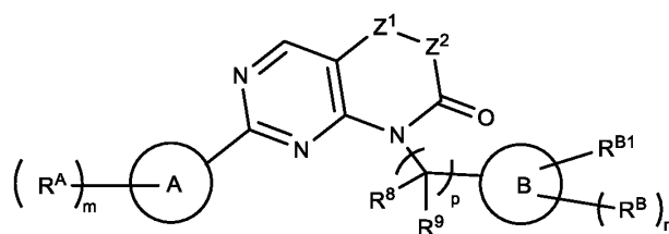
Formula (IIIa-2),
