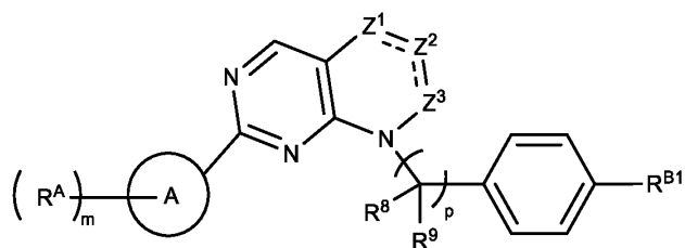
Formula (IIIc-1).
