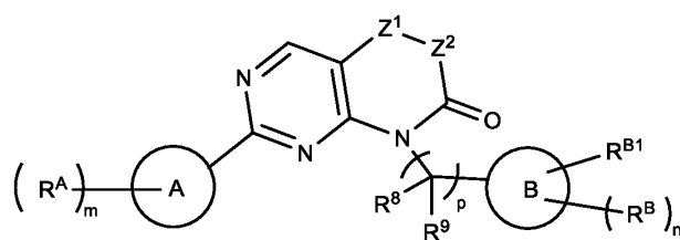
Formula (IIIa-2)
