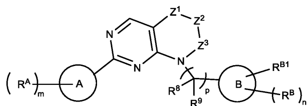
Formula (IIIb),
