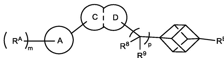
Formula (VI)
