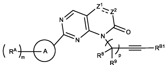
Formula (IIId').
