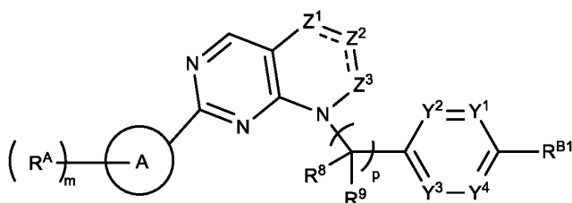
Formula (IIIc)
