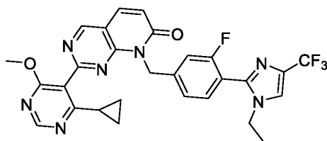
Compound 24
