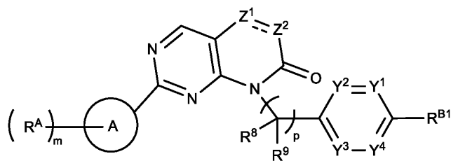
Formula (IIIc')
