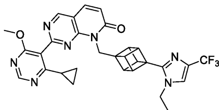
Compound 25
