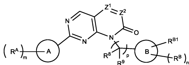
Formula (IIIa-1),
