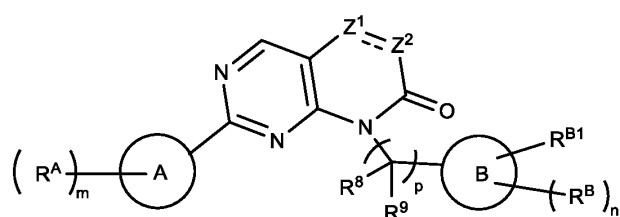
Formula (IIIa)
