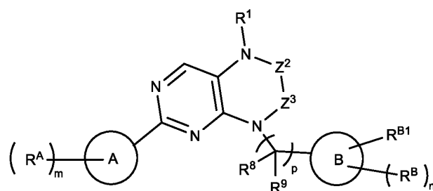
Formula (IIIb-2)
