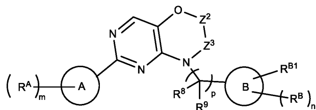
Formula (IIIb-1)
