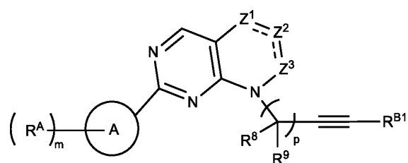
Formula (IIIId).
