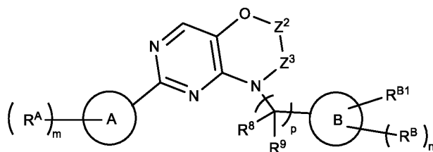
Formula (IIIb-1),
