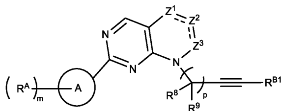
Formula (IIIId),
