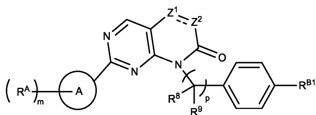
Formula (IIIc-1').
