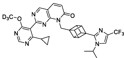
Compound 32
