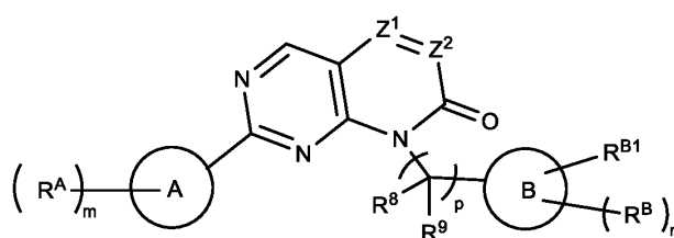
Formula (IIIa-1),
