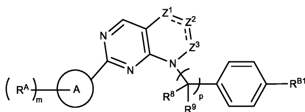
Formula (IIIc-1).
