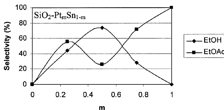
FIG. 1A - Selectivity Pt/Sn Catalyst
