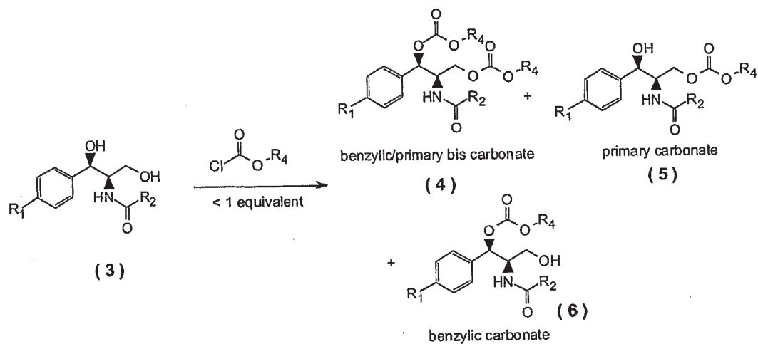
FIG. 2B (Scheme 4)
