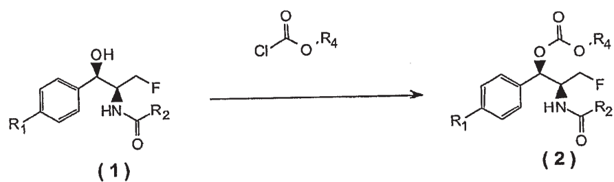
FIG. 1A (Scheme 1)
