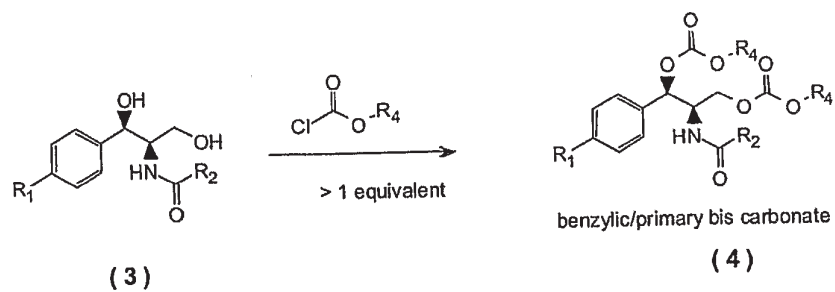
FIG. 1B (Scheme 2)
