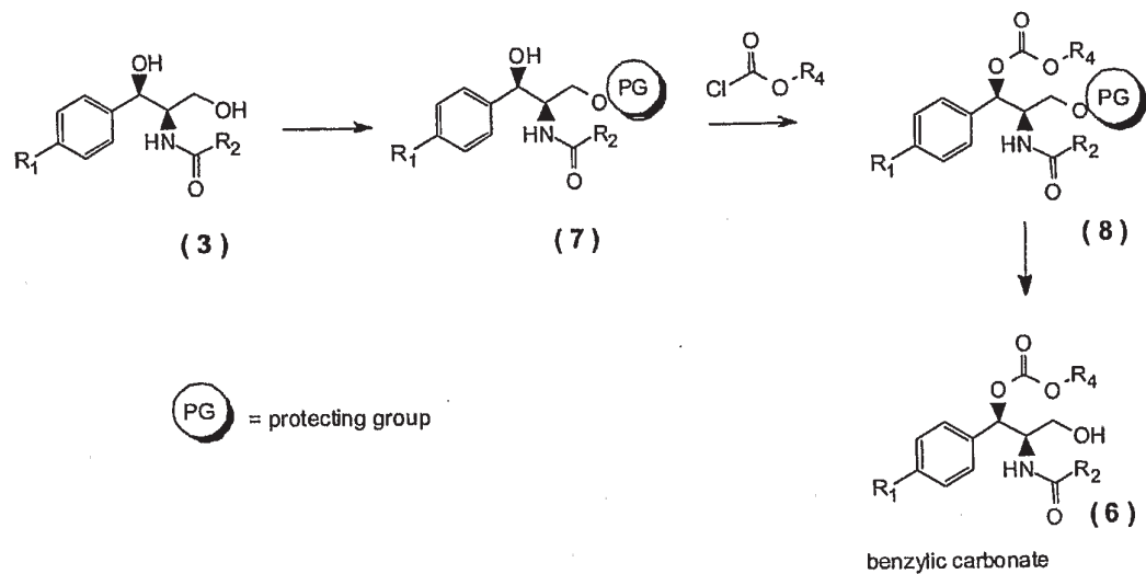
FIG. 2B (Scheme 4)
