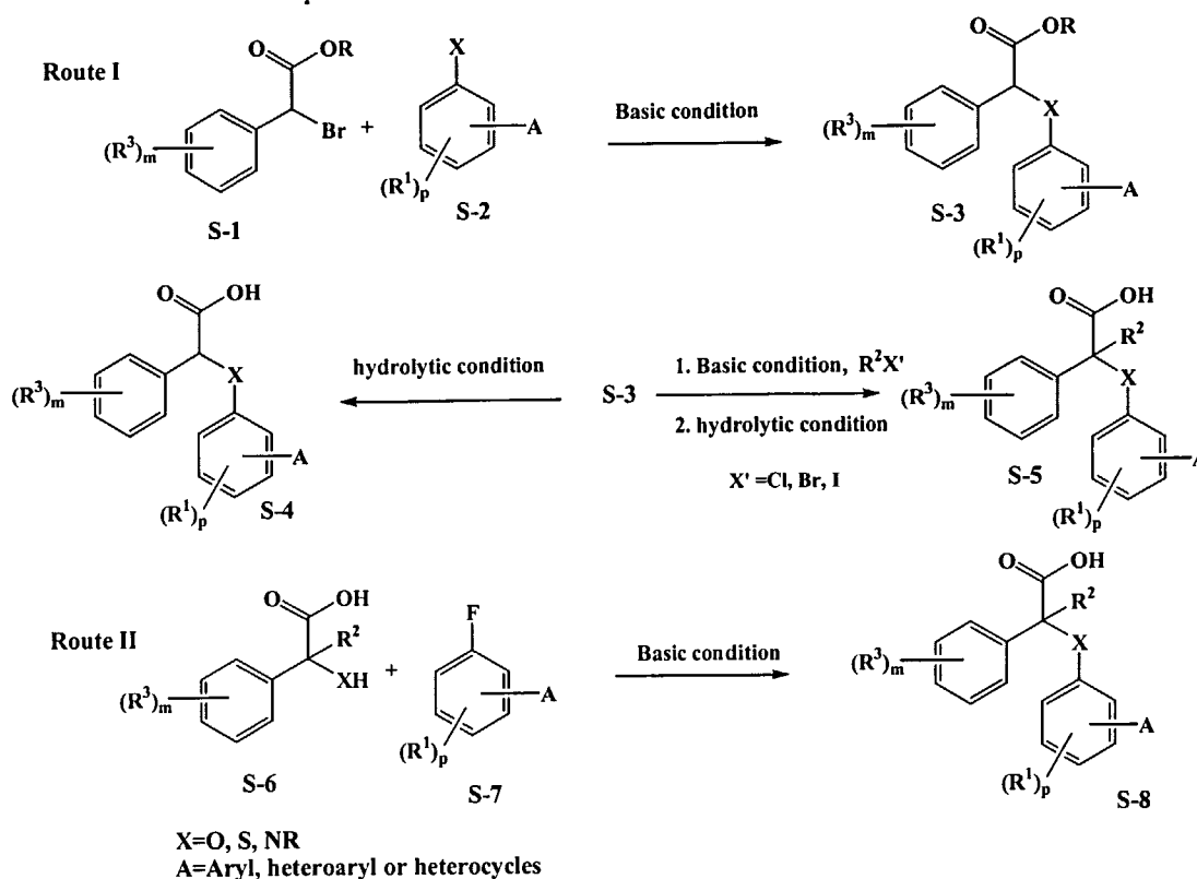
Figure 1. General Reaction Schemes
