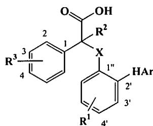
Compound XII and XIIa
