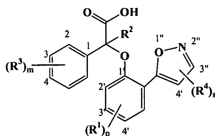
Compounds IX and IXa
