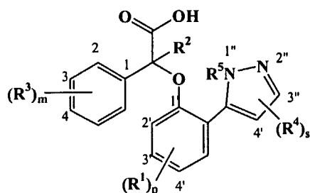
Compounds X and Xa
