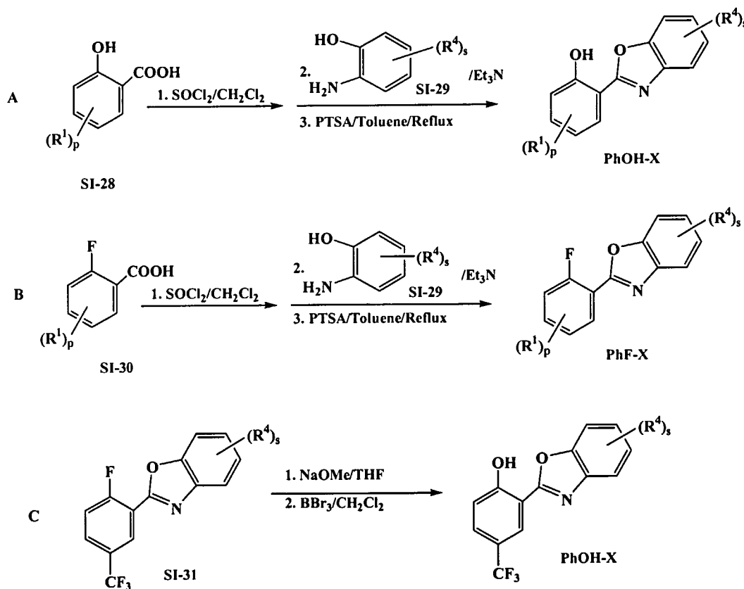
Scheme 2 Synthesis of 2-benzooxazol-2-yl-phenols and 2-benzooxazol-2-yl-phenylfluorides
