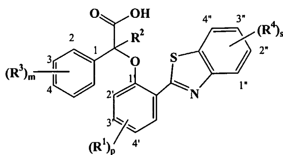
Compounds II and IIa
