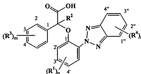
Compound XI and XIa
