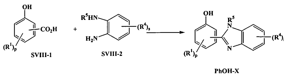
Scheme 6. Synthesis of benzoimidazol-2-yl-phenols
