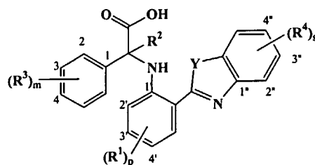
Compounds VI and VIa
