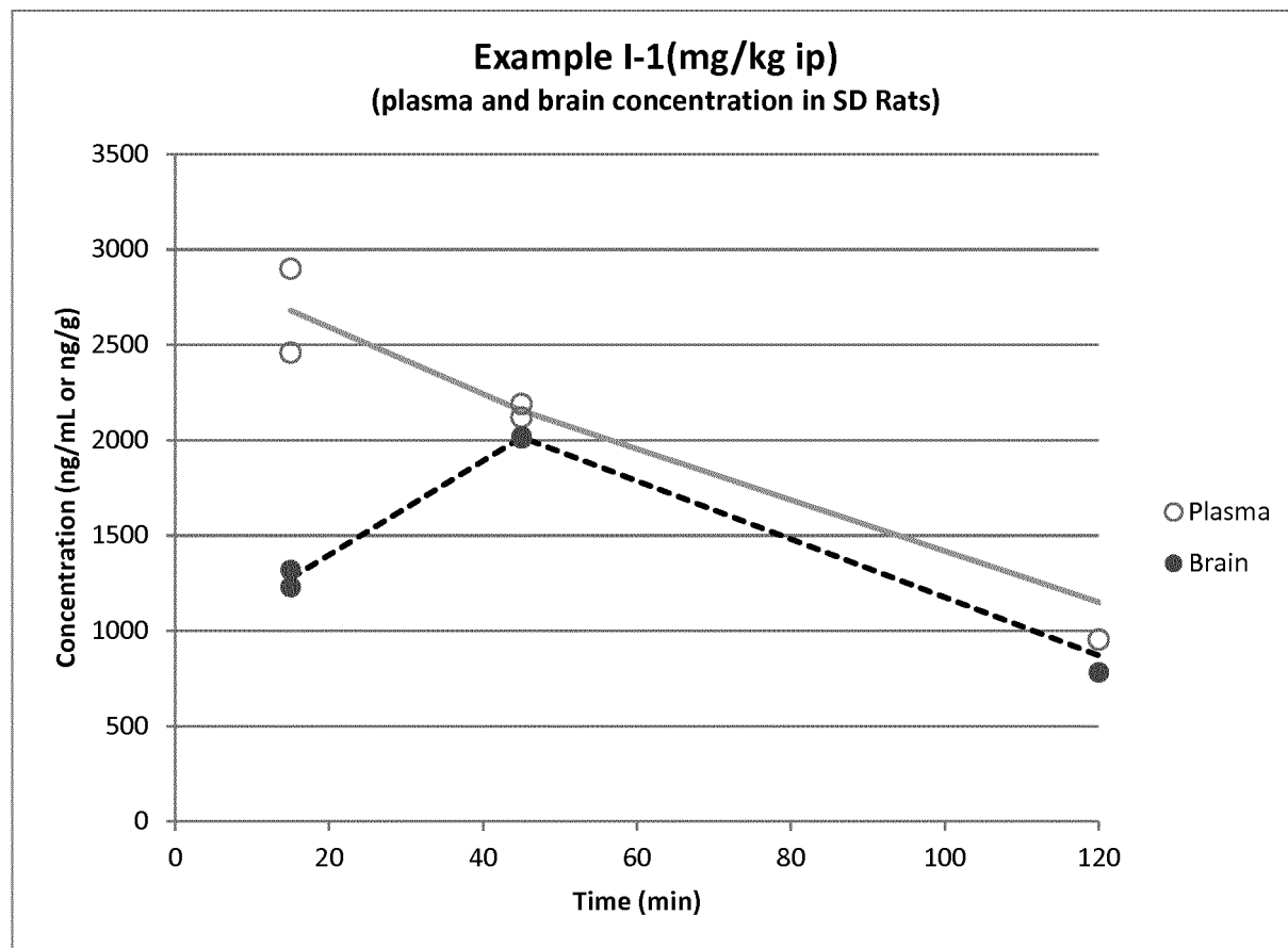
Figure 3: Plasma and brain exposure levels of Example compound I-1
