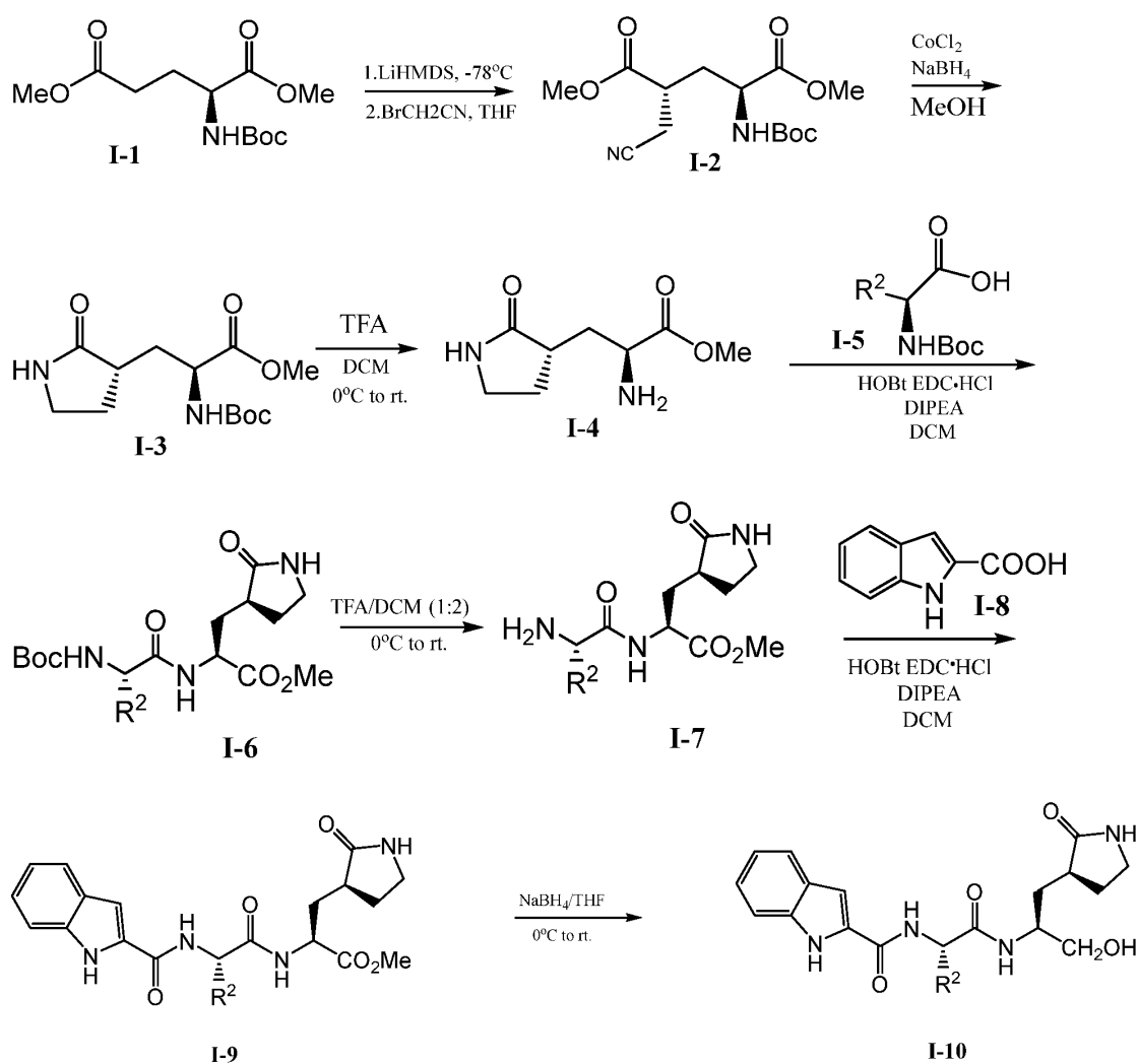
Scheme I. General methods for making aldehyde intermediates for compounds of Formula (I).
