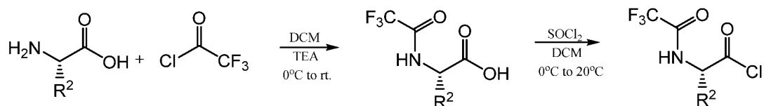
Scheme III. Synthesis methods for compounds of Formula (II).
