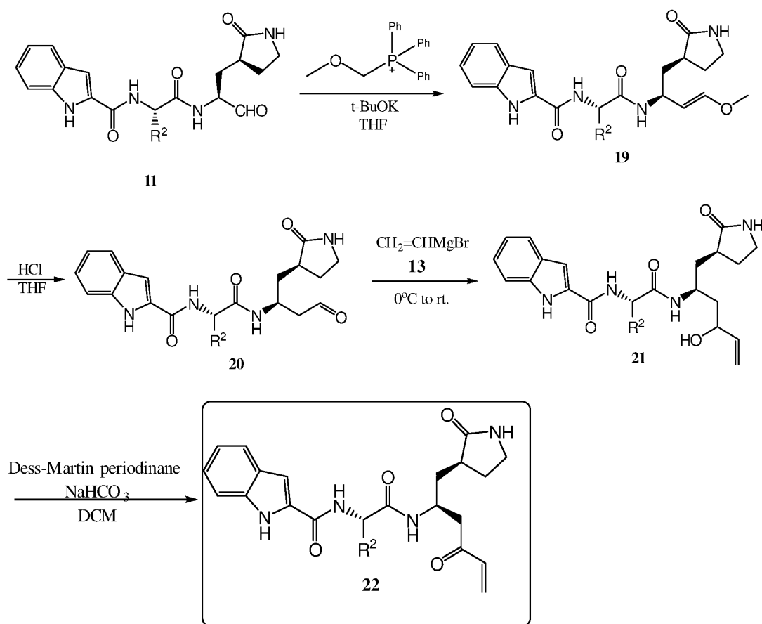
Scheme V. Additional synthesis methods for compounds of Formula (I).
