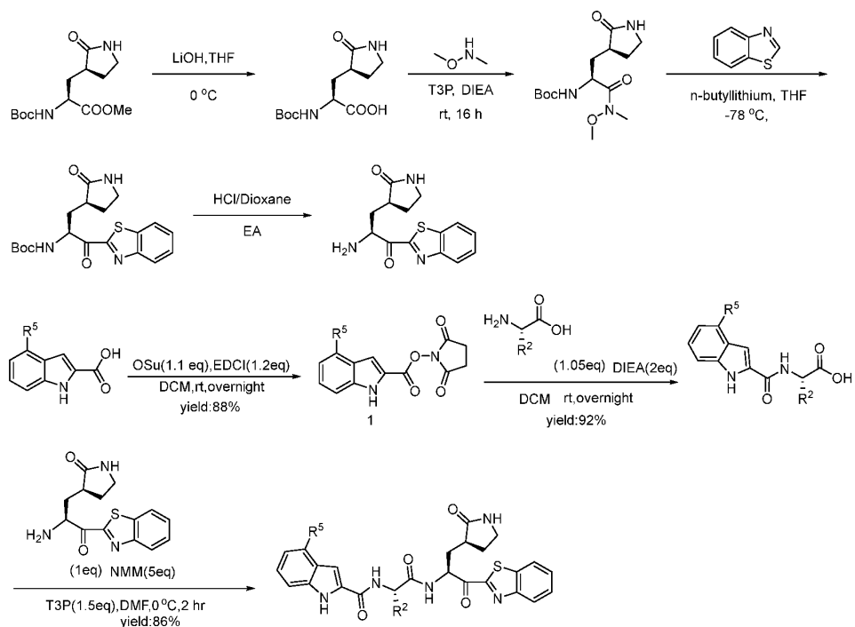
Scheme X. Synthesis of selected compounds of Formula (I).
