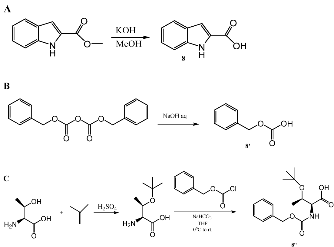
Scheme II. Synthesis of selected precursors.
