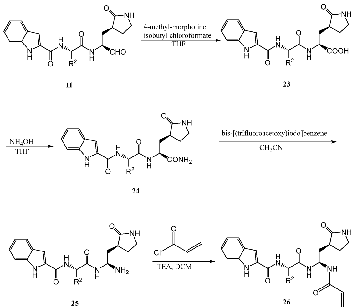
Scheme VI. Synthesis of selected compounds of Formula (I).
