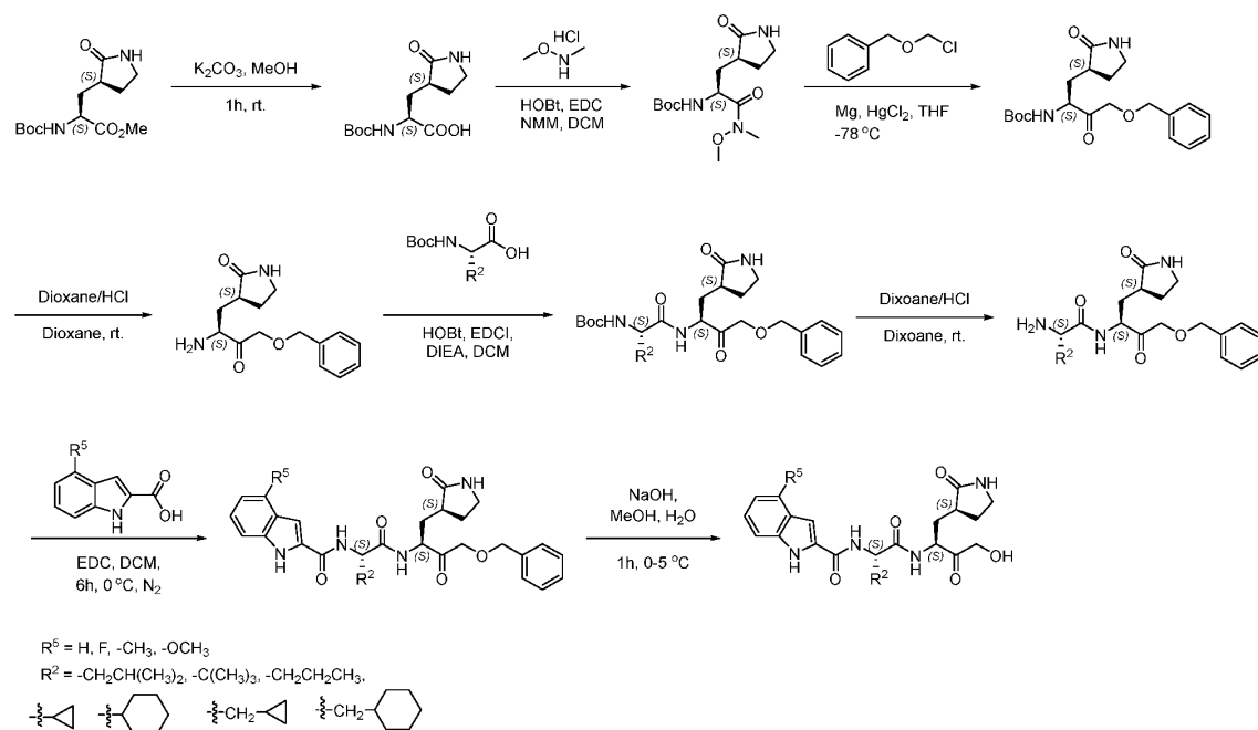
Scheme VIII. Synthesis of selected compounds of Formula (II).
