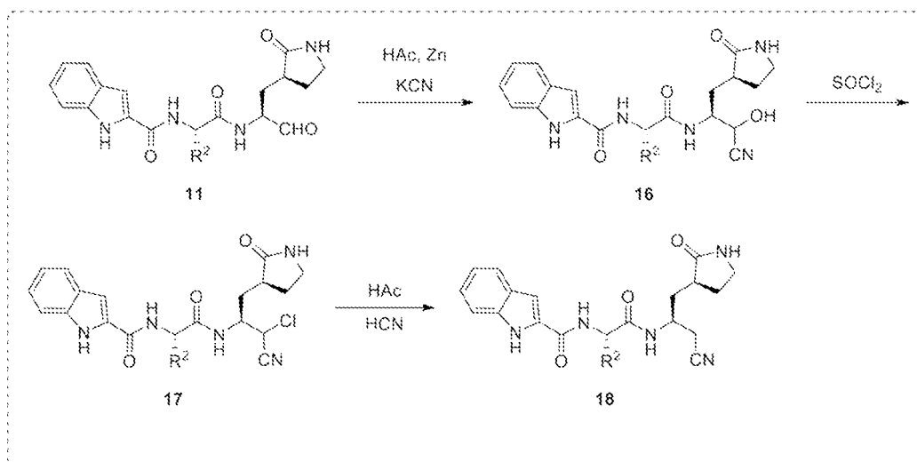
Scheme V. Additional synthesis methods for compounds of Formula (I).
