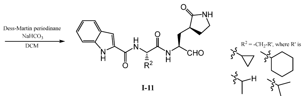
Scheme II. Synthesis of selected precursors.
