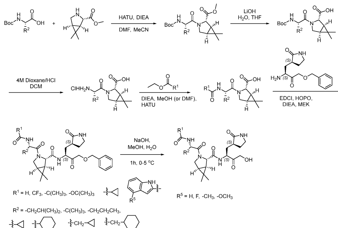
Scheme VIII. Synthesis of selected compounds of Formula (II).
