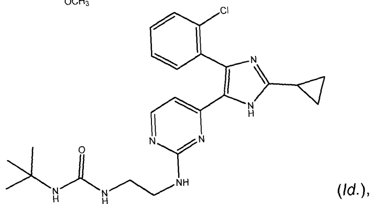
Compound 26
