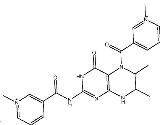
Compound 7
