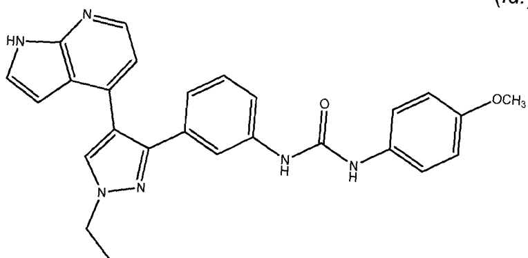
Compound 33
