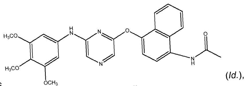
Compound 25
