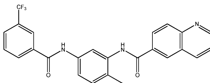
Compound 16 ( Id. ),
