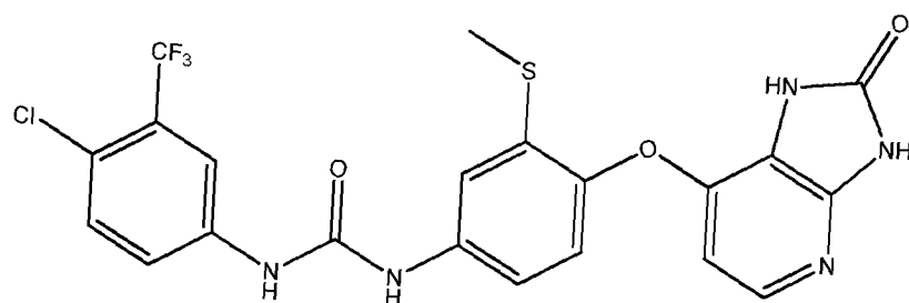
Compound 37
