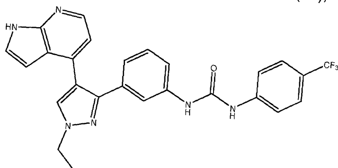
Compound 32
