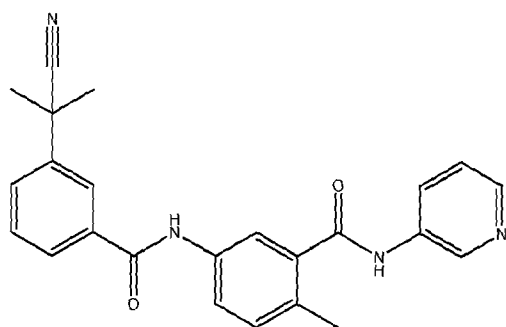
Compound 20
