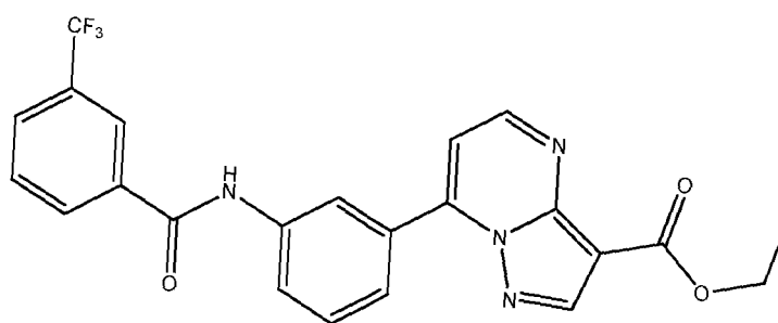
Compound 38
