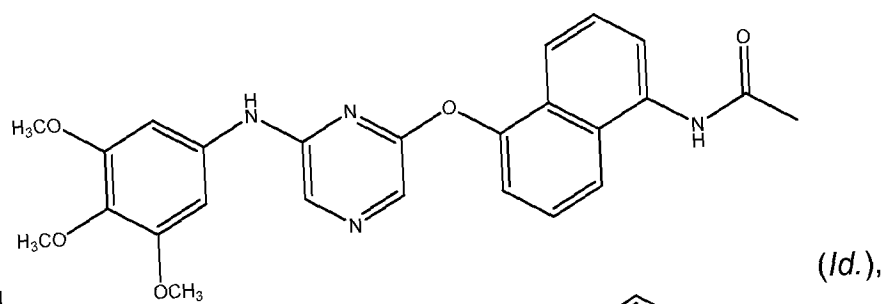
Compound 24
