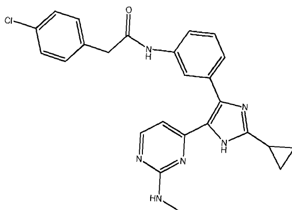
Compound 31
