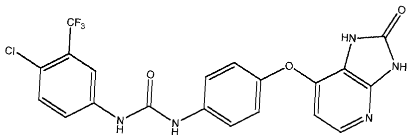
Compound 34
