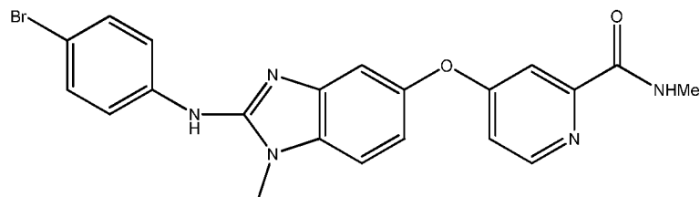
Compound 16 ( Id. ),
