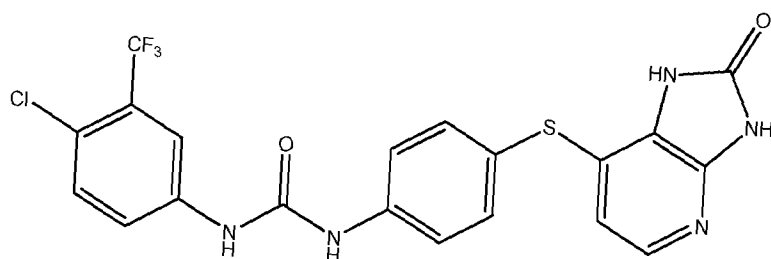
Compound 36
