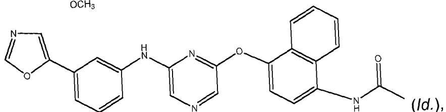
Compound 24
