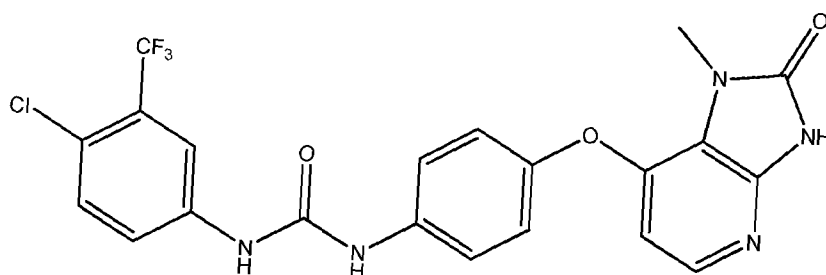
Compound 35 (Id.),
