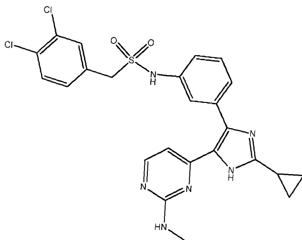
Compound 30
