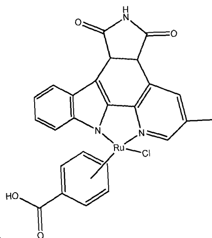
Compound 13
