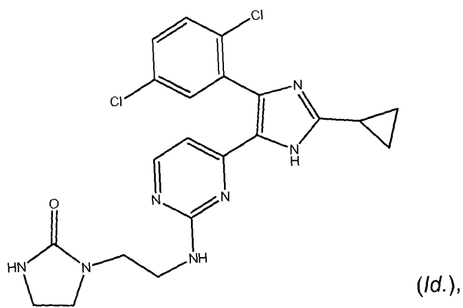
Compound 28
