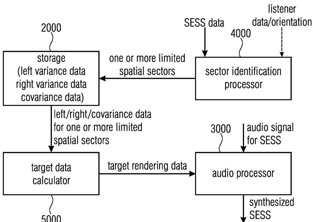
Fig. 3 (THIRD ASPECT)
