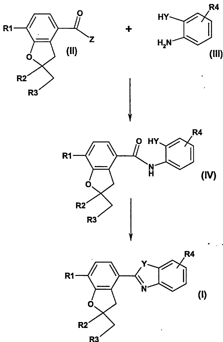
Scheme 1
