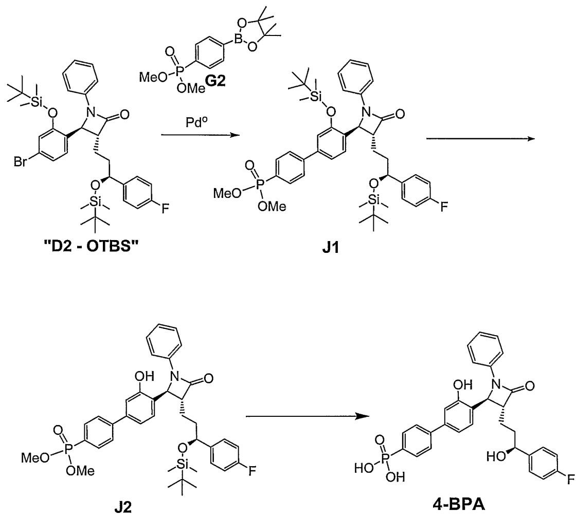
Scheme 6
