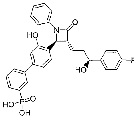
3-BPA
