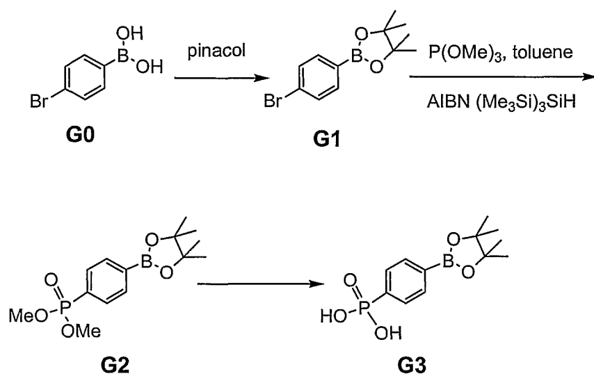
Scheme 3b
