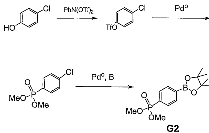
Scheme 3a
