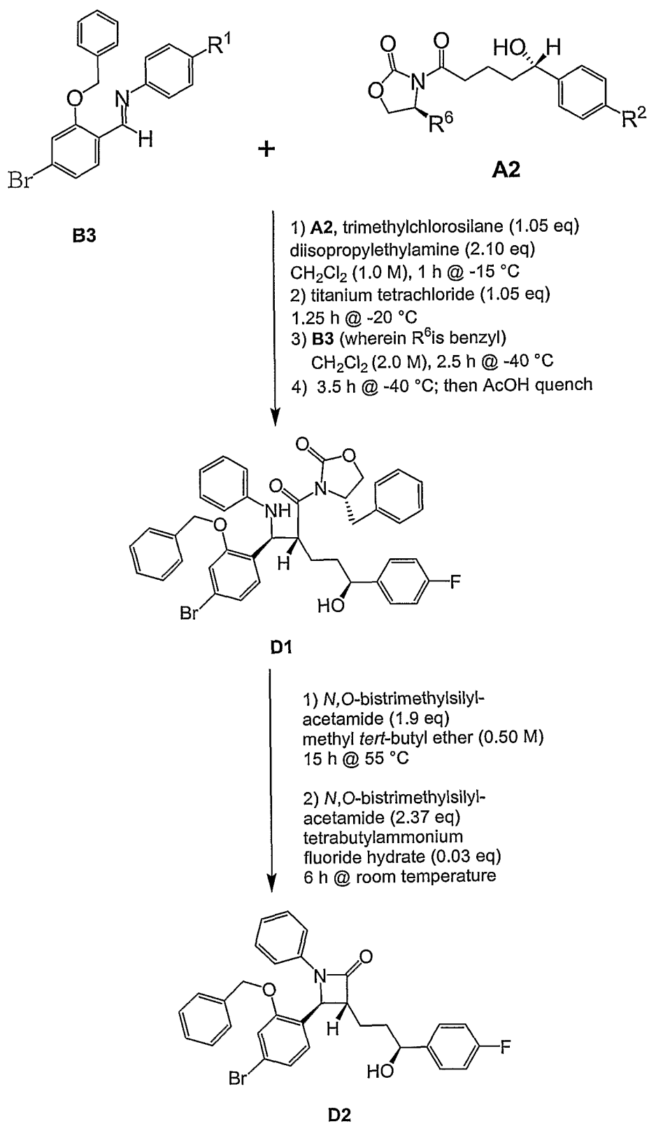
Scheme 4
