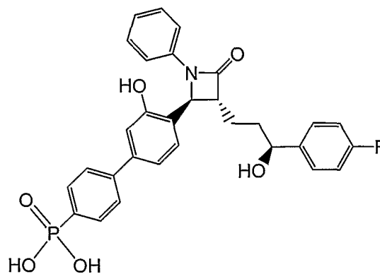
4-BPA
