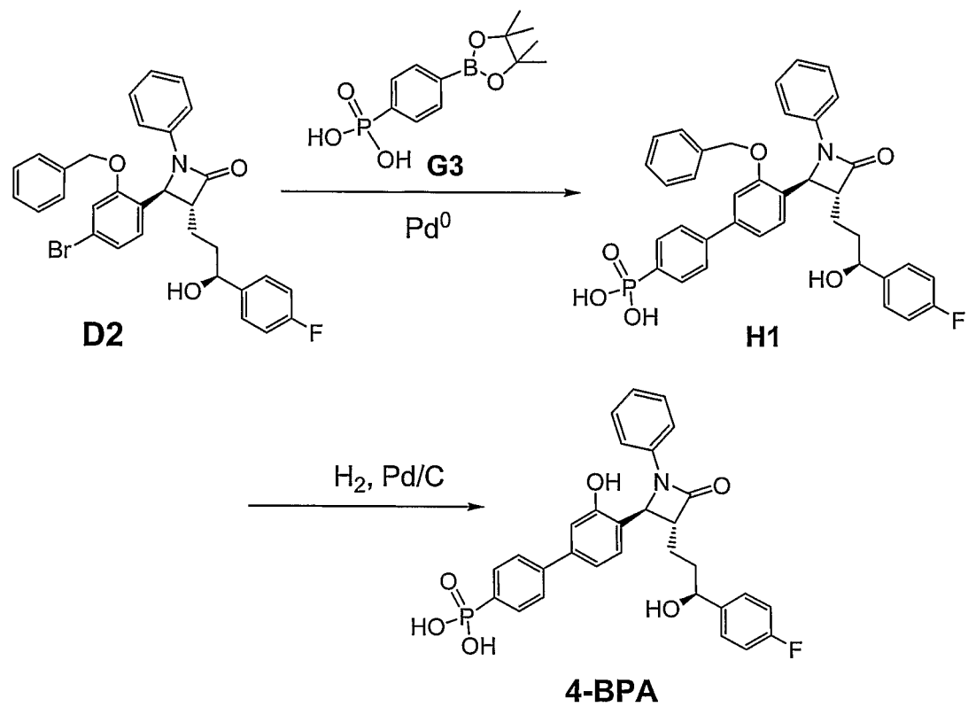
Scheme 7
