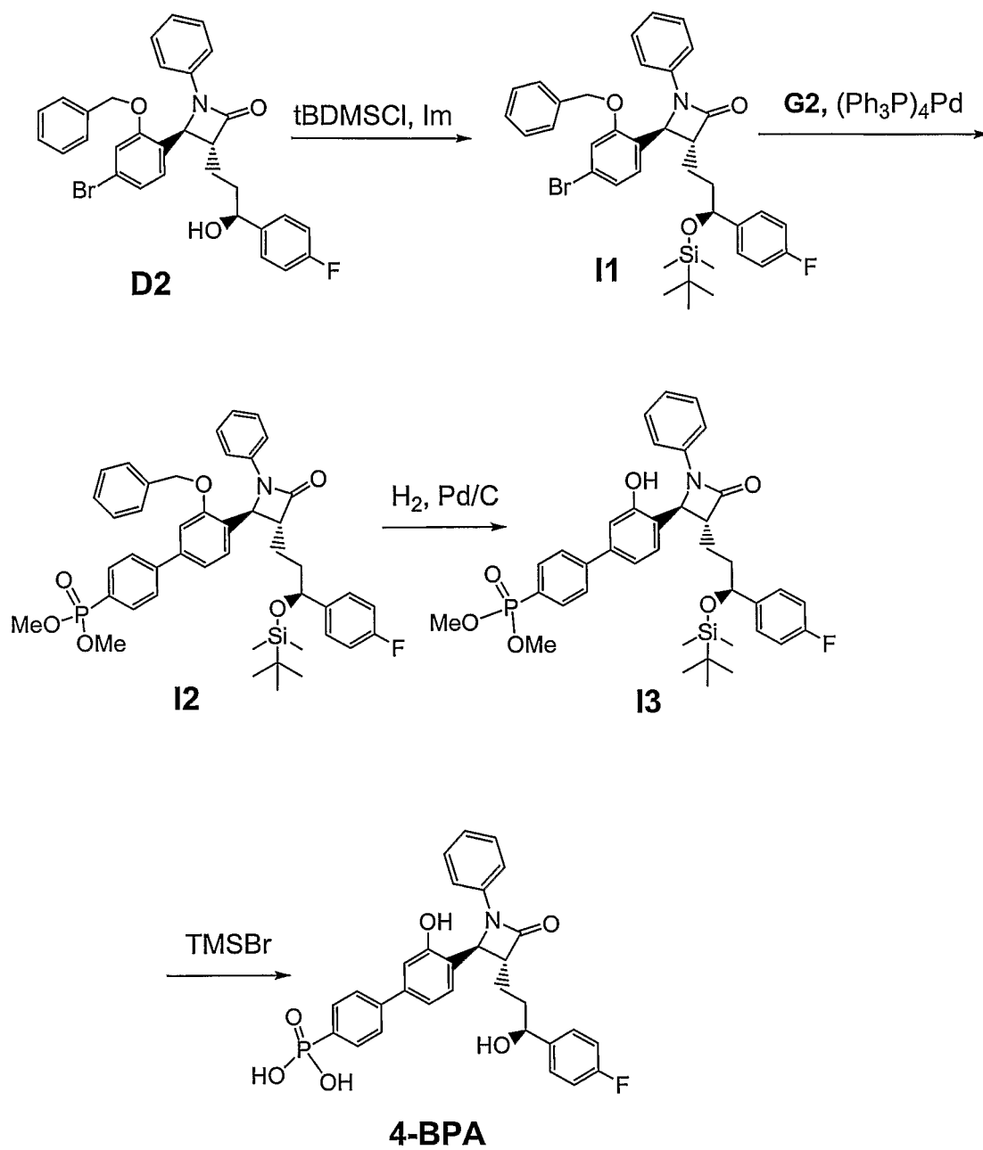
Scheme 5
