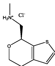
(S)-TPMA HCl
