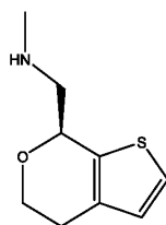
(S)-TPMA.
