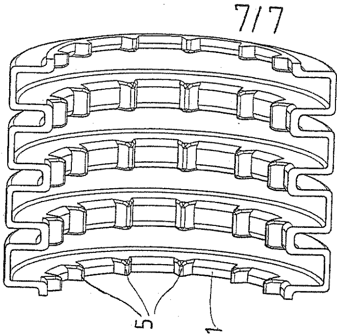
Isometric view Scale 5:1
