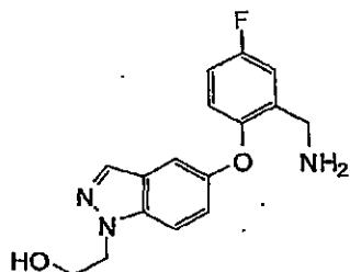
2-(5-(2-(Aminomethyl)-4-fluorophenoxy)-1H-indazol-1-yl)ethanol (79A)
