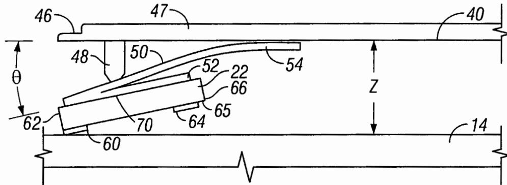
FIG. 3 (Prior Art)
