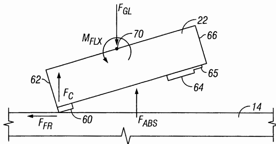
FIG. 4 (Prior Art)
