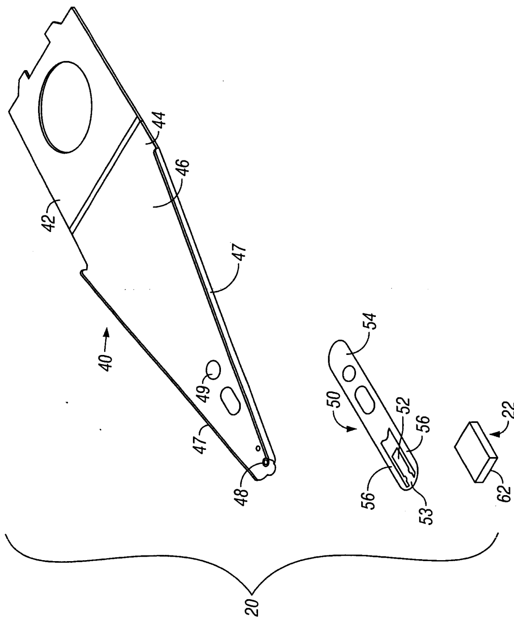
FIG. 2 (Prior Art)
