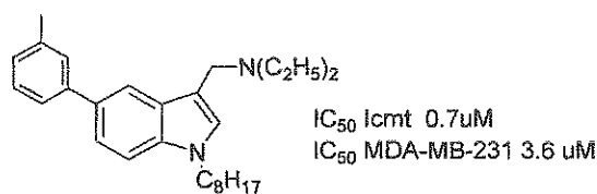
N-ethyl-N-[(1-octyl-5-m-tolyl-1H-indol-3-yl)methyl]ethanamine
