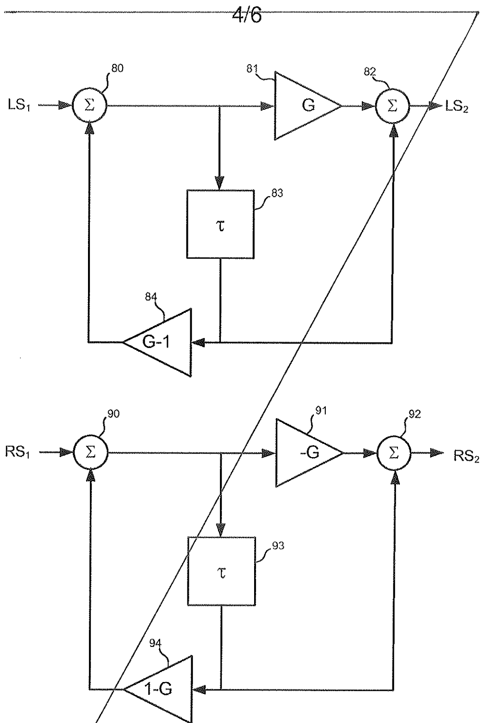
Figure 5 – Decorrelation Filters
