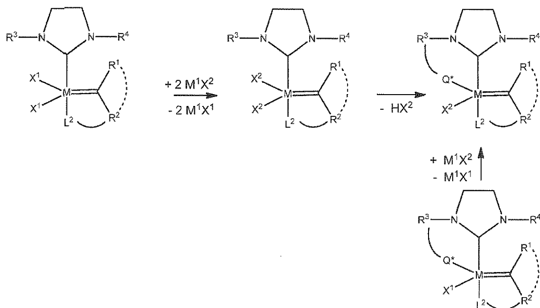
Scheme 3. Synthetic Procedure
