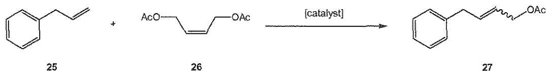
Scheme 14
