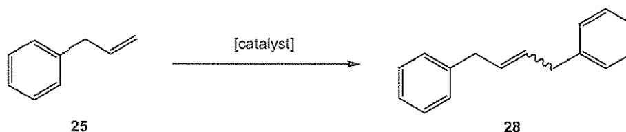
Scheme 15
