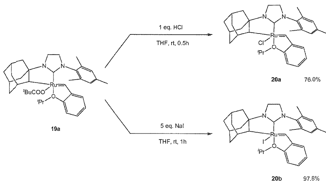
Scheme 10
