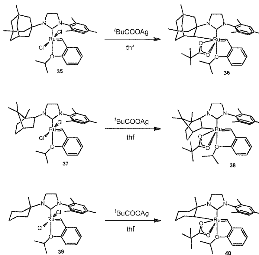
Scheme 20
