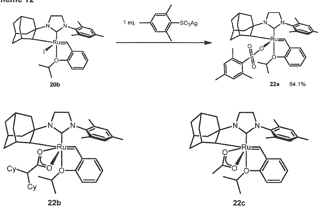
Scheme 12
