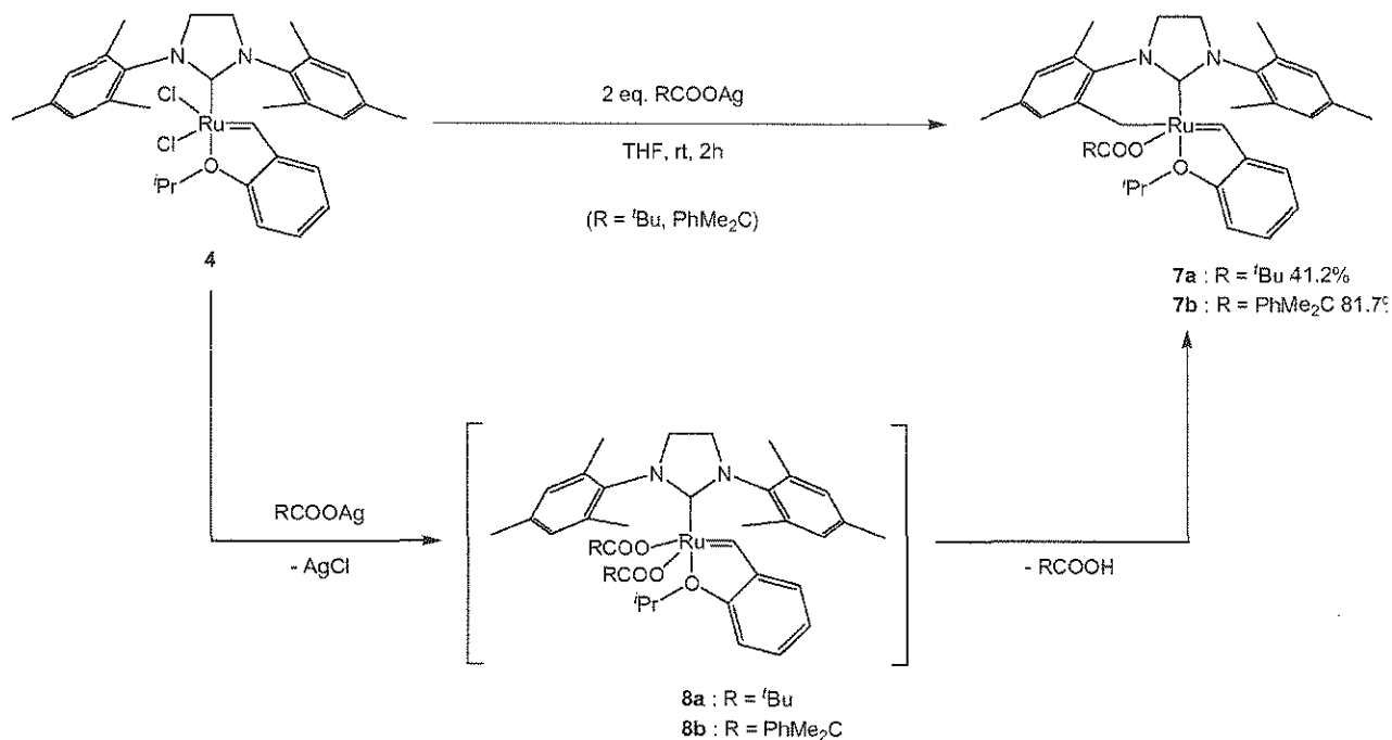
Scheme 4
