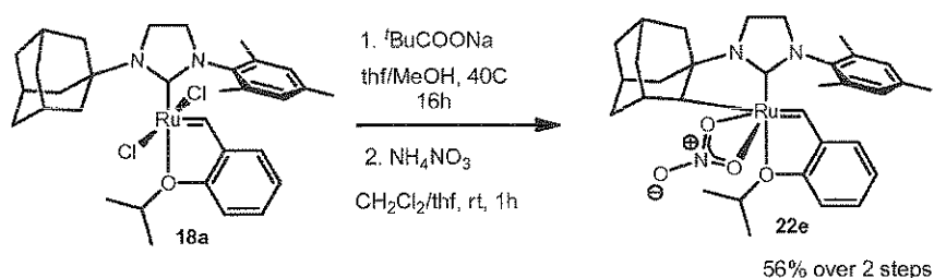
Scheme 18
