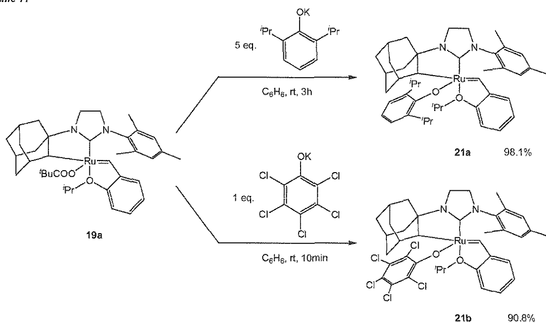
Scheme 11
