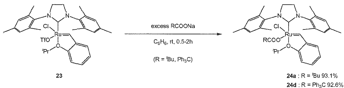
Scheme 13
