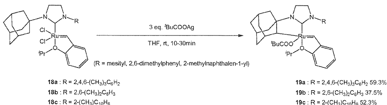
Scheme 9
