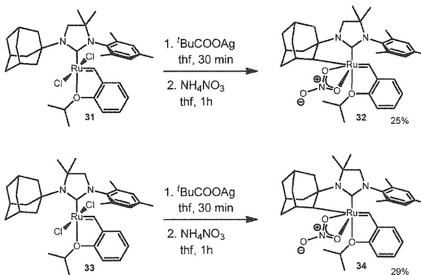
Scheme 19
