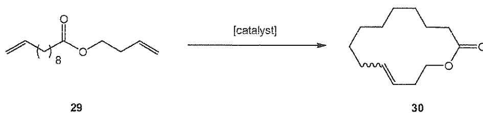
Scheme 16
