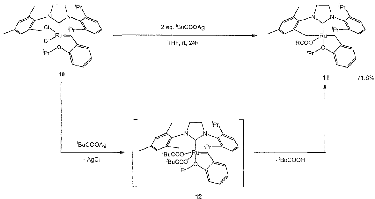
Scheme 6
