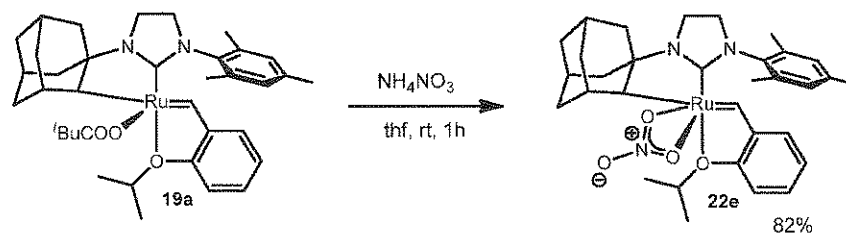
Scheme 18
