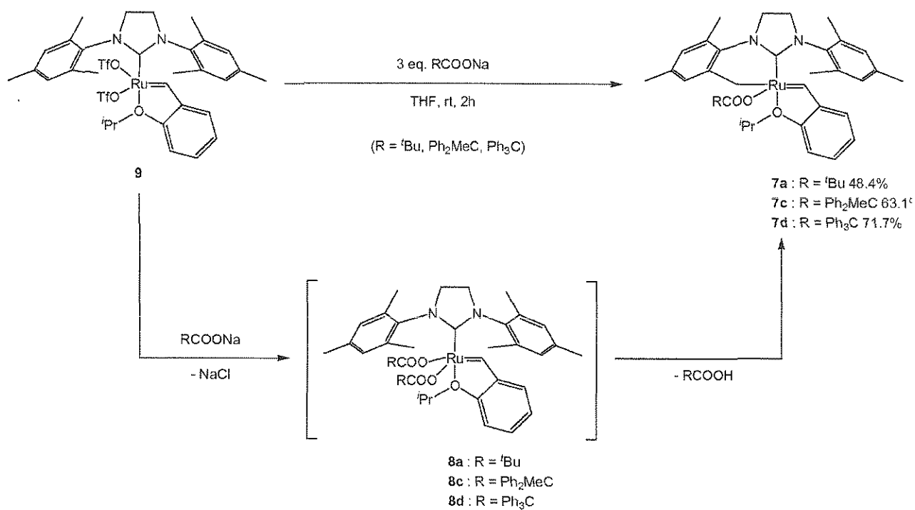
Scheme 5
