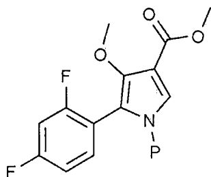
[Chemical Formula 1-6]
