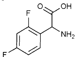
[Chemical Formula 1-3]
