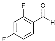
[Chemical Formula 1-2]
