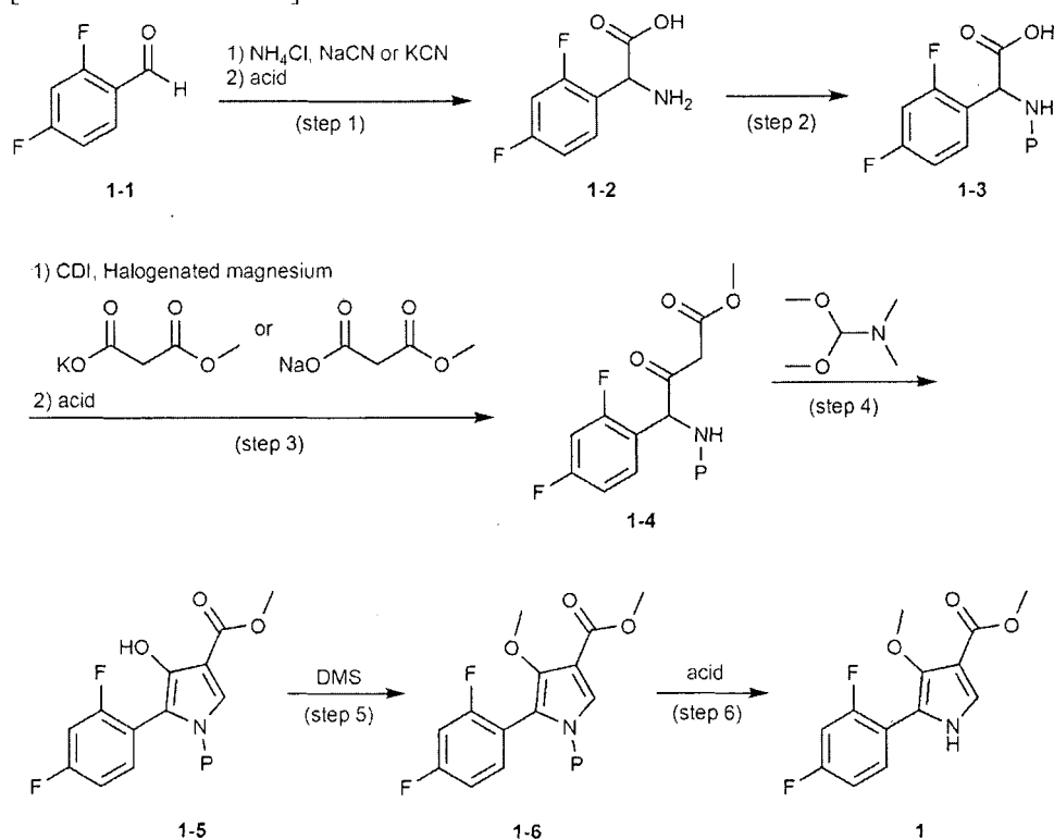
[Reaction Scheme 1]
