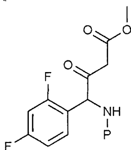
[Chemical Formula 1-5]
