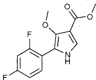
[Chemical Formula 1-1]
