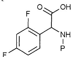
[Chemical Formula 1-4]
