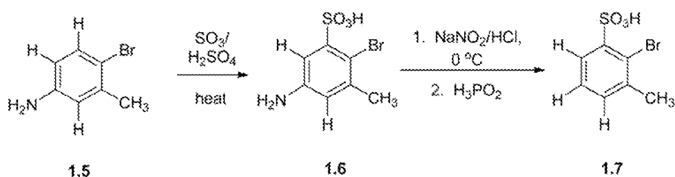
Scheme 1B.
