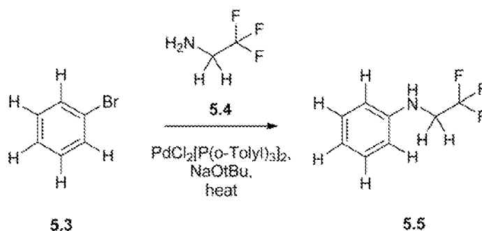
Scheme 5B.
