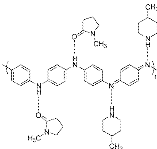
SCHEME III.
