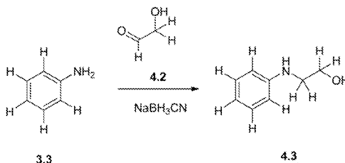
Scheme 4B.
