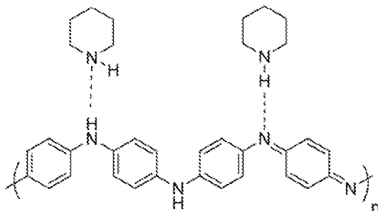
SCHEME II.
