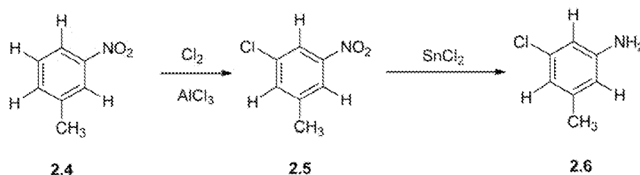
Scheme 2B.
