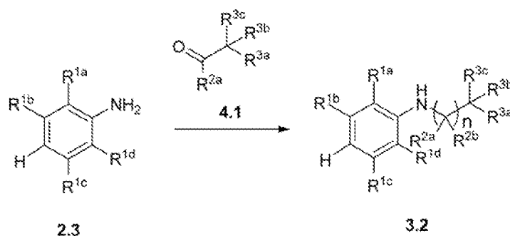
Scheme 4A.
