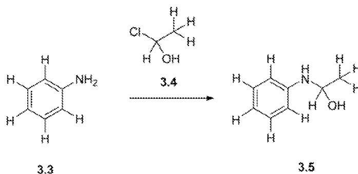
Scheme 3B.
