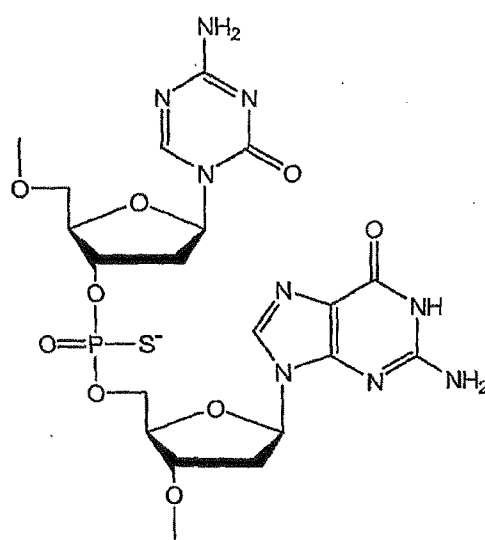
-DpG- Islet with Phosphorothioate Backbone
