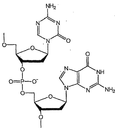
-DpG- Islet with Natural Phosphodiester Backbone
