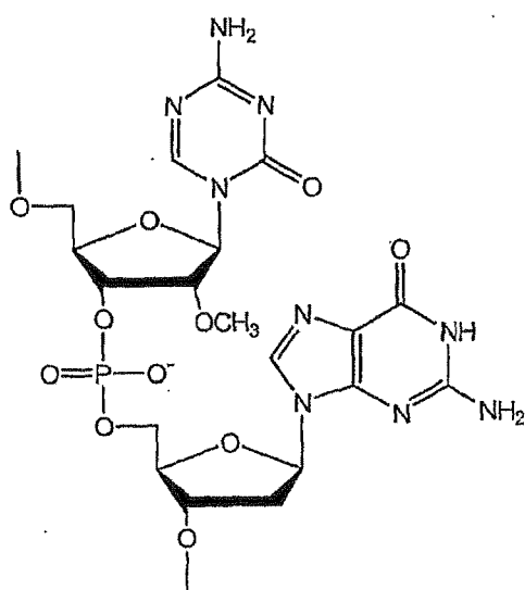
-DpG- Islet with 2'-Methoxy Ribose Phosphodiester Backbone
