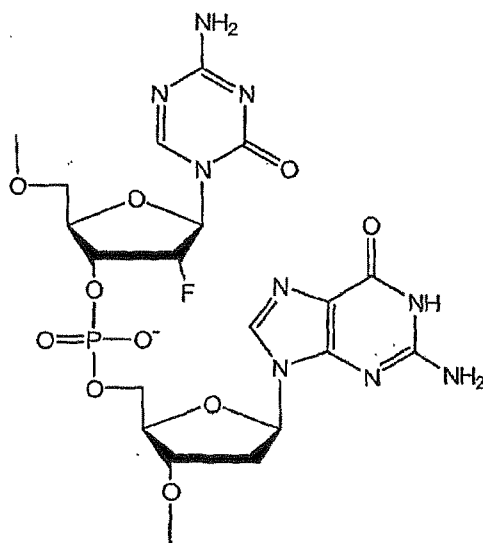
-DpG- Islet with 2'-Fluoro Ribose Phosphodiester Backbone
