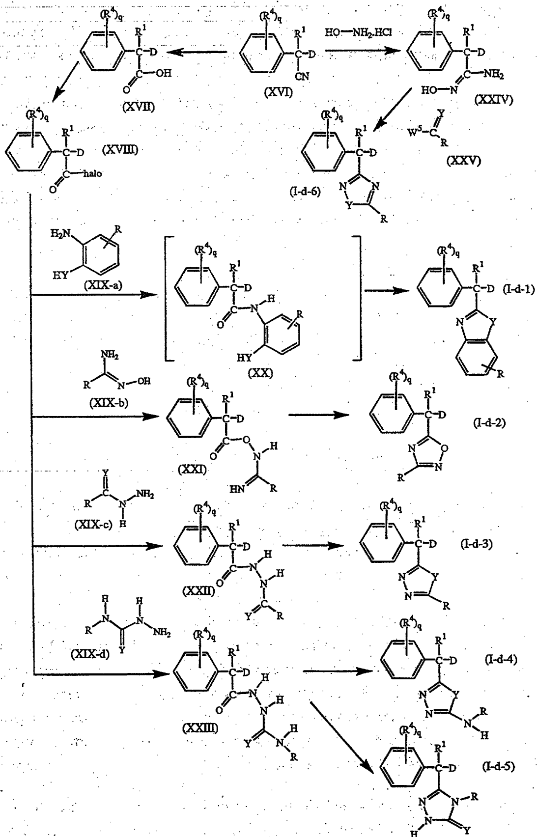
Scheme 3
