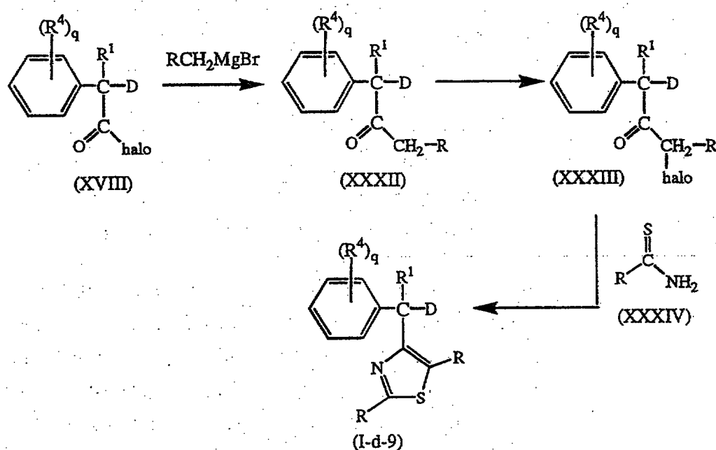
Scheme 5
