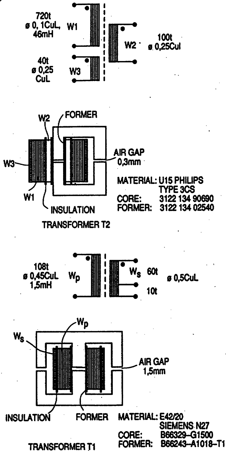
FIG. 4 TRANSFORMER DATA
