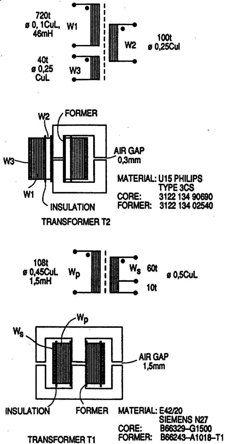
FIG. 4 TRANSFORMER DATA
