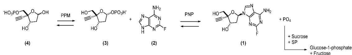
Scheme II. Overall Reaction Scheme to Produce Compound (1)
