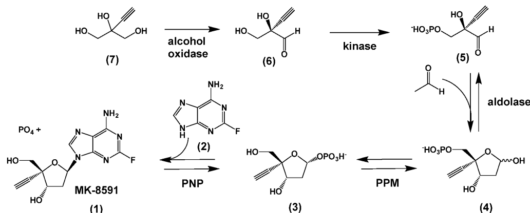
Scheme I. Production of MK-8591
