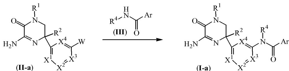
Reaction Scheme 1
